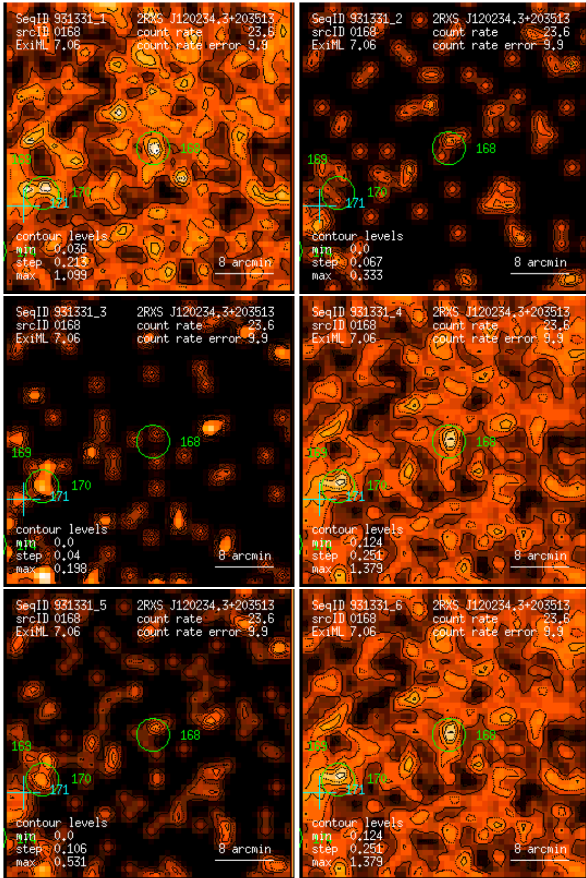
Figure 168: RASS 931331: detection 0168: band rate images, Gaussian filter: (1) PSPC channels 11 – 41, (2) 52 – 90, (3) 91 – 201, (4) 11 – 235, (5) 52 – 201, (6) 11 – 201. Broad band rates in counts/ks. Band rate contour levels in counts/ks/arcmin 2 .
