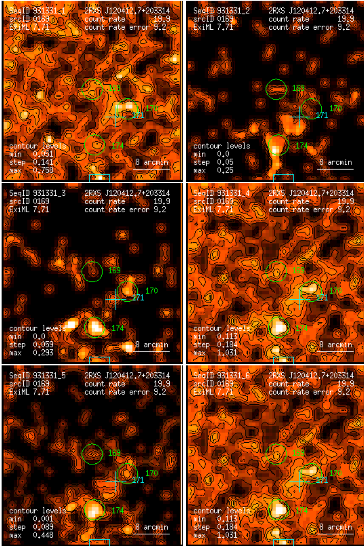
Figure 169: RASS 931331: detection 0169: band rate images, Gaussian filter: (1) PSPC channels 11 – 41, (2) 52 – 90, (3) 91 – 201, (4) 11 – 235, (5) 52 – 201, (6) 11 – 201. Broad band rates in counts/ks. Band rate contour levels in counts/ks/arcmin 2 .
