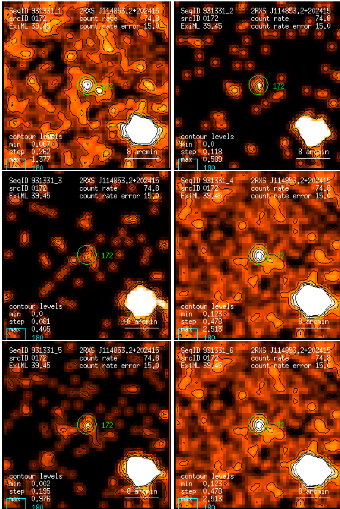
Figure 172: RASS 931331: detection 0172: band rate images, Gaussian filter: (1) PSPC channels 11 – 41, (2) 52 – 90, (3) 91 – 201, (4) 11 – 235, (5) 52 – 201, (6) 11 – 201. Broad band rates in counts/ks. Band rate contour levels in counts/ks/arcmin 2 .
