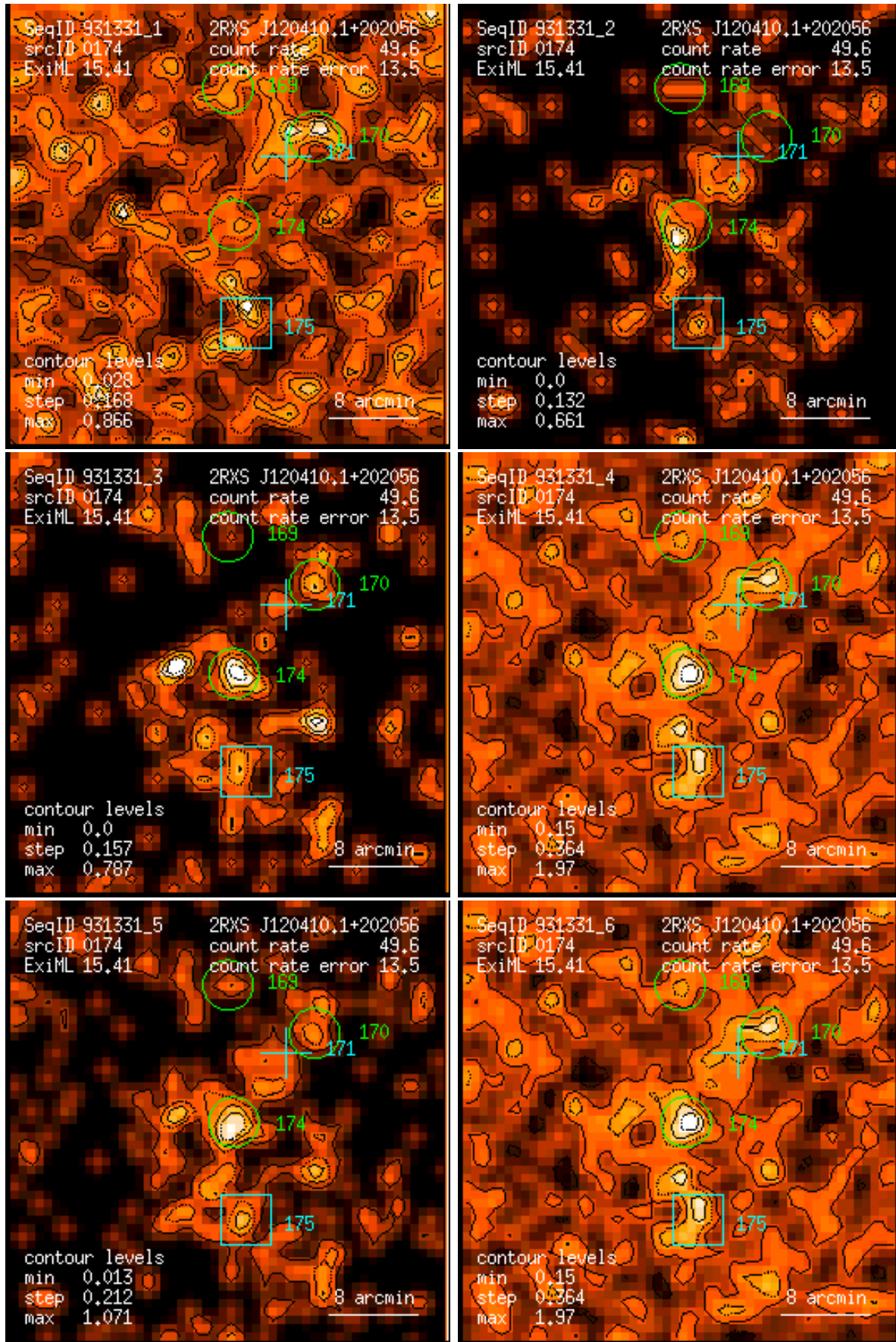
Figure 174: RASS 931331: detection 0174: band rate images, Gaussian filter: (1) PSPC channels 11 – 41, (2) 52 – 90, (3) 91 – 201, (4) 11 – 235, (5) 52 – 201, (6) 11 – 201. Broad band rates in counts/ks. Band rate contour levels in counts/ks/arcmin 2 .
