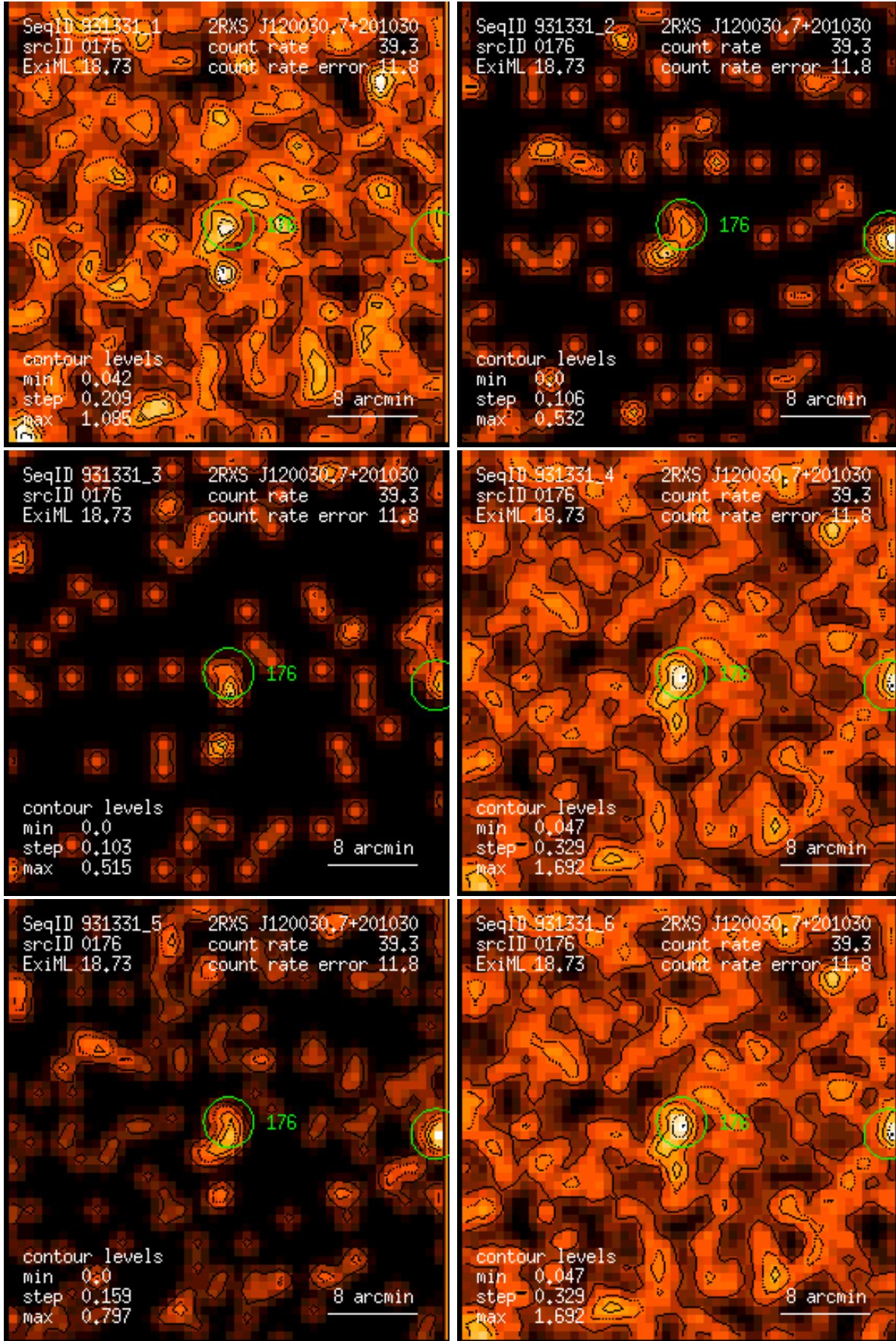
Figure 176: RASS 931331: detection 0176: band rate images, Gaussian filter: (1) PSPC channels 11 – 41, (2) 52 – 90, (3) 91 – 201, (4) 11 – 235, (5) 52 – 201, (6) 11 – 201. Broad band rates in counts/ks. Band rate contour levels in counts/ks/arcmin 2 .
