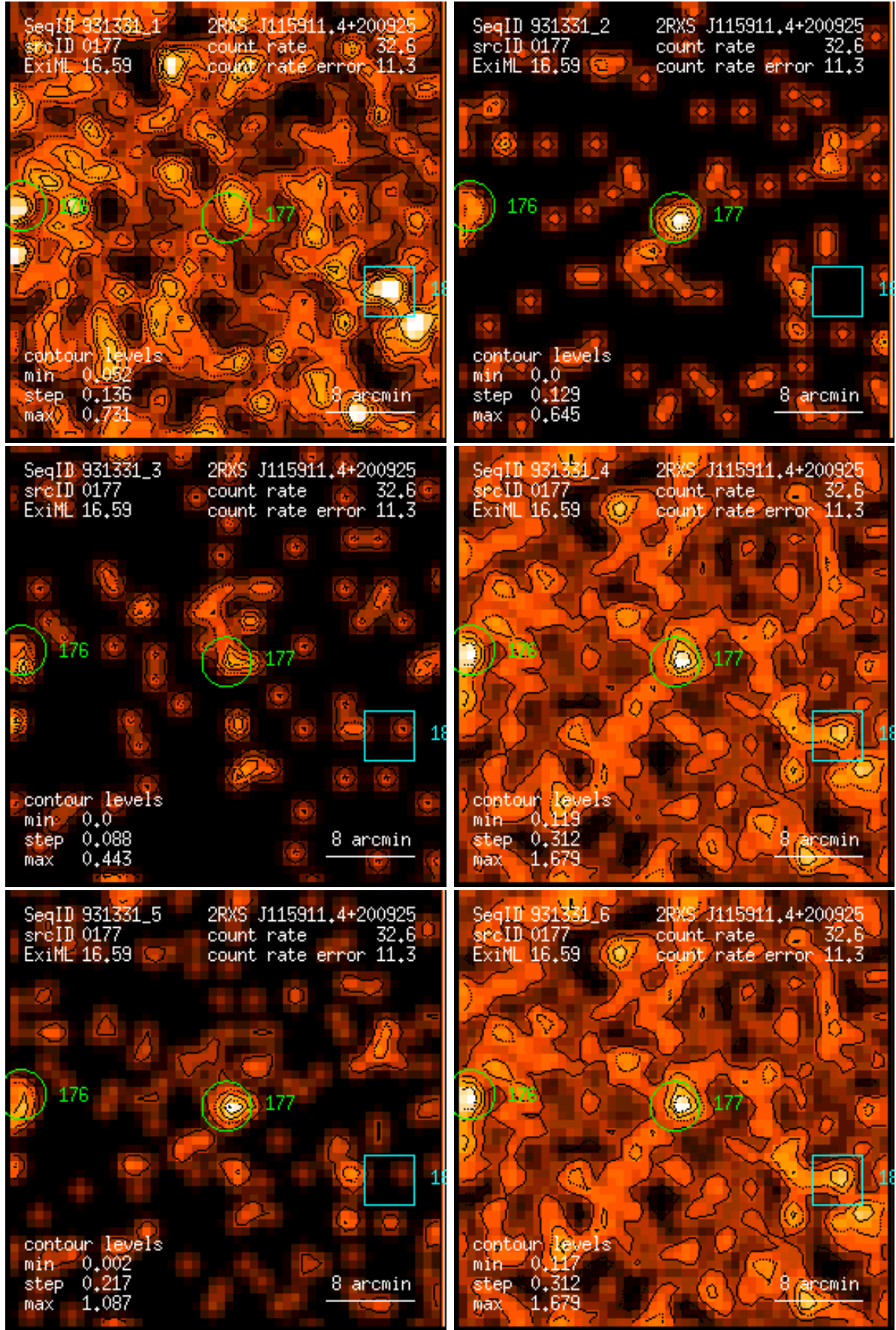
Figure 177: RASS 931331: detection 0177: band rate images, Gaussian filter: (1) PSPC channels 11 – 41, (2) 52 – 90, (3) 91 – 201, (4) 11 – 235, (5) 52 – 201, (6) 11 – 201. Broad band rates in counts/ks. Band rate contour levels in counts/ks/arcmin 2 .
