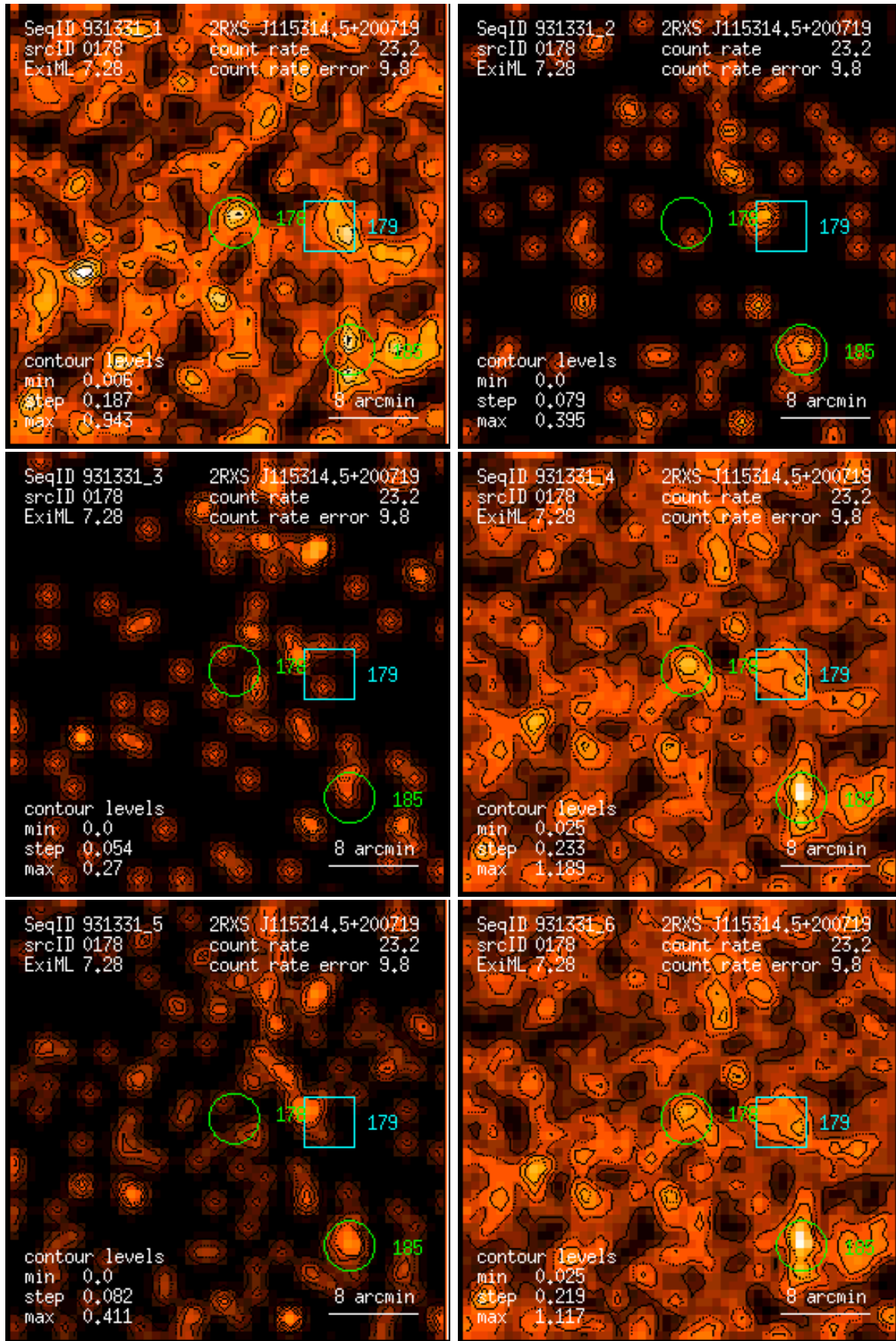
Figure 178: RASS 931331: detection 0178: band rate images, Gaussian filter: (1) PSPC channels 11 – 41, (2) 52 – 90, (3) 91 – 201, (4) 11 – 235, (5) 52 – 201, (6) 11 – 201. Broad band rates in counts/ks. Band rate contour levels in counts/ks/arcmin 2 .
