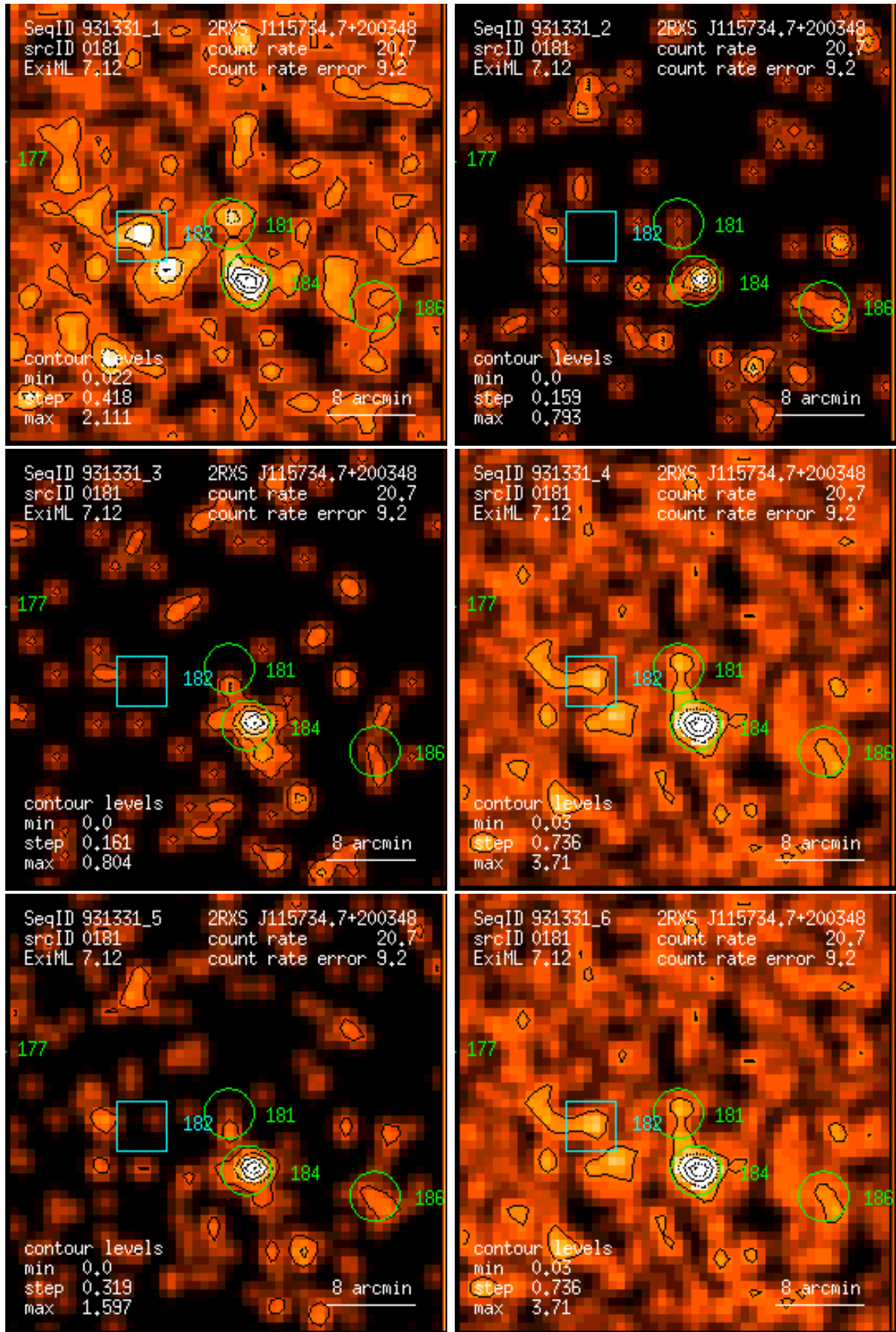
Figure 181: RASS 931331: detection 0181: band rate images, Gaussian filter: (1) PSPC channels 11 – 41, (2) 52 – 90, (3) 91 – 201, (4) 11 – 235, (5) 52 – 201, (6) 11 – 201. Broad band rates in counts/ks. Band rate contour levels in counts/ks/arcmin 2 .
