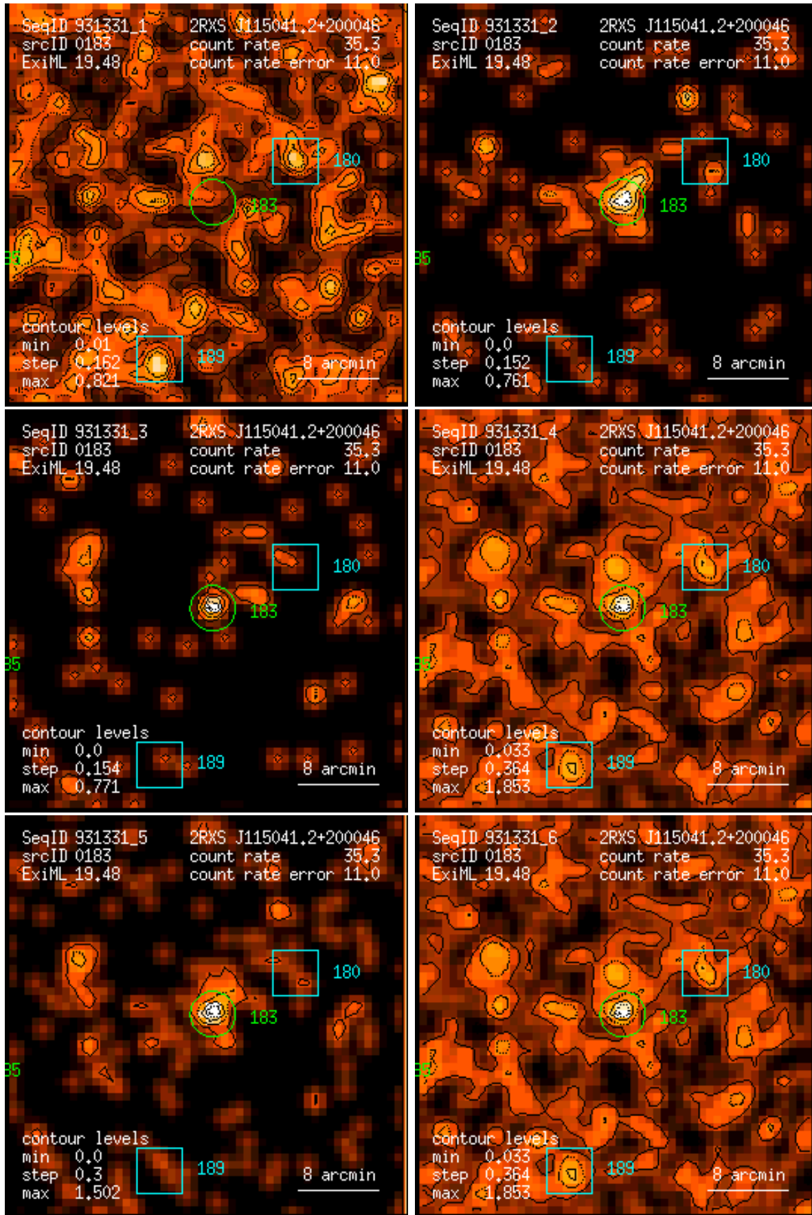
Figure 183: RASS 931331: detection 0183: band rate images, Gaussian filter: (1) PSPC channels 11 – 41, (2) 52 – 90, (3) 91 – 201, (4) 11 – 235, (5) 52 – 201, (6) 11 – 201. Broad band rates in counts/ks. Band rate contour levels in counts/ks/arcmin 2 .
