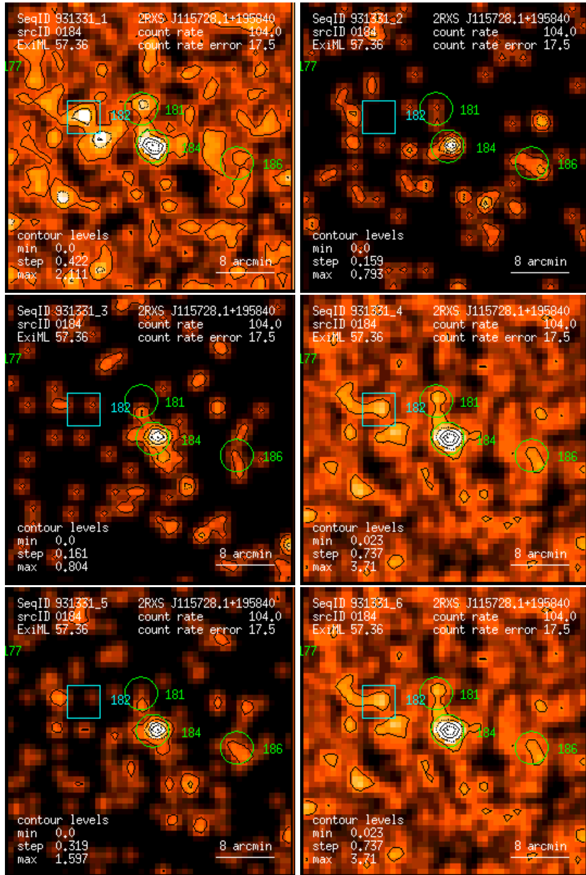
Figure 184: RASS 931331: detection 0184: band rate images, Gaussian filter: (1) PSPC channels 11 – 41, (2) 52 – 90, (3) 91 – 201, (4) 11 – 235, (5) 52 – 201, (6) 11 – 201. Broad band rates in counts/ks. Band rate contour levels in counts/ks/arcmin 2 .
