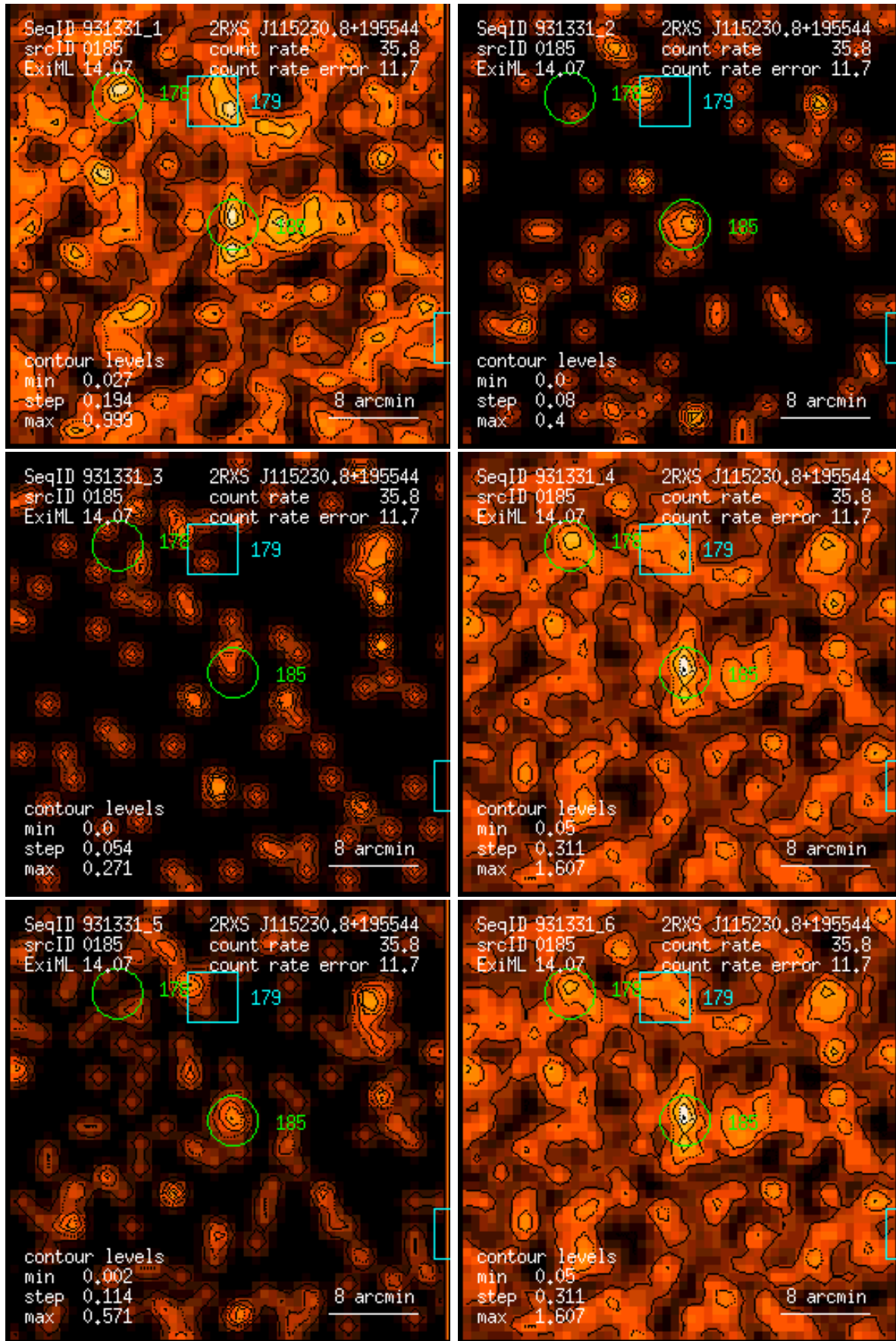
Figure 185: RASS 931331: detection 0185: band rate images, Gaussian filter: (1) PSPC channels 11 – 41, (2) 52 – 90, (3) 91 – 201, (4) 11 – 235, (5) 52 – 201, (6) 11 – 201. Broad band rates in counts/ks. Band rate contour levels in counts/ks/arcmin 2 .
