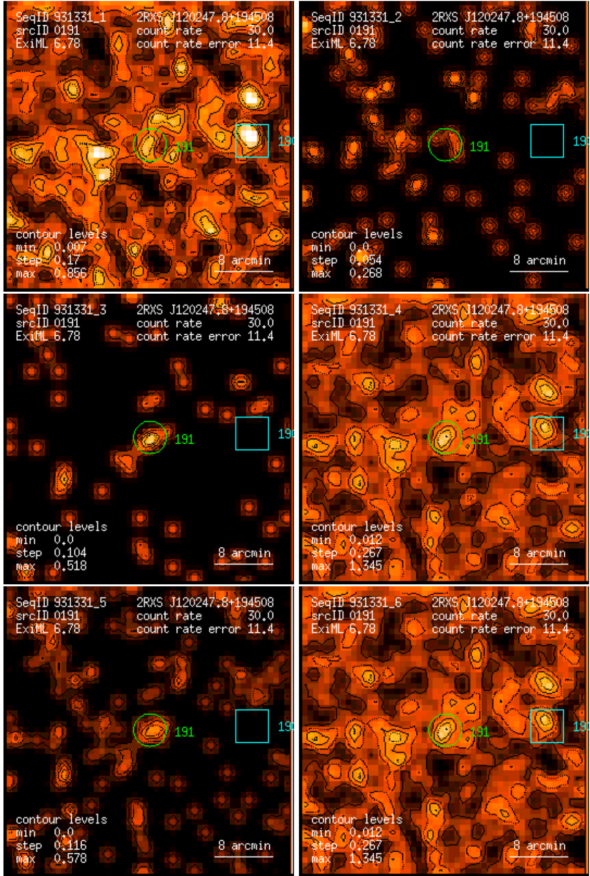
Figure 191: RASS 931331: detection 0191: band rate images, Gaussian filter: (1) PSPC channels 11 – 41, (2) 52 – 90, (3) 91 – 201, (4) 11 – 235, (5) 52 – 201, (6) 11 – 201. Broad band rates in counts/ks. Band rate contour levels in counts/ks/arcmin 2 .
