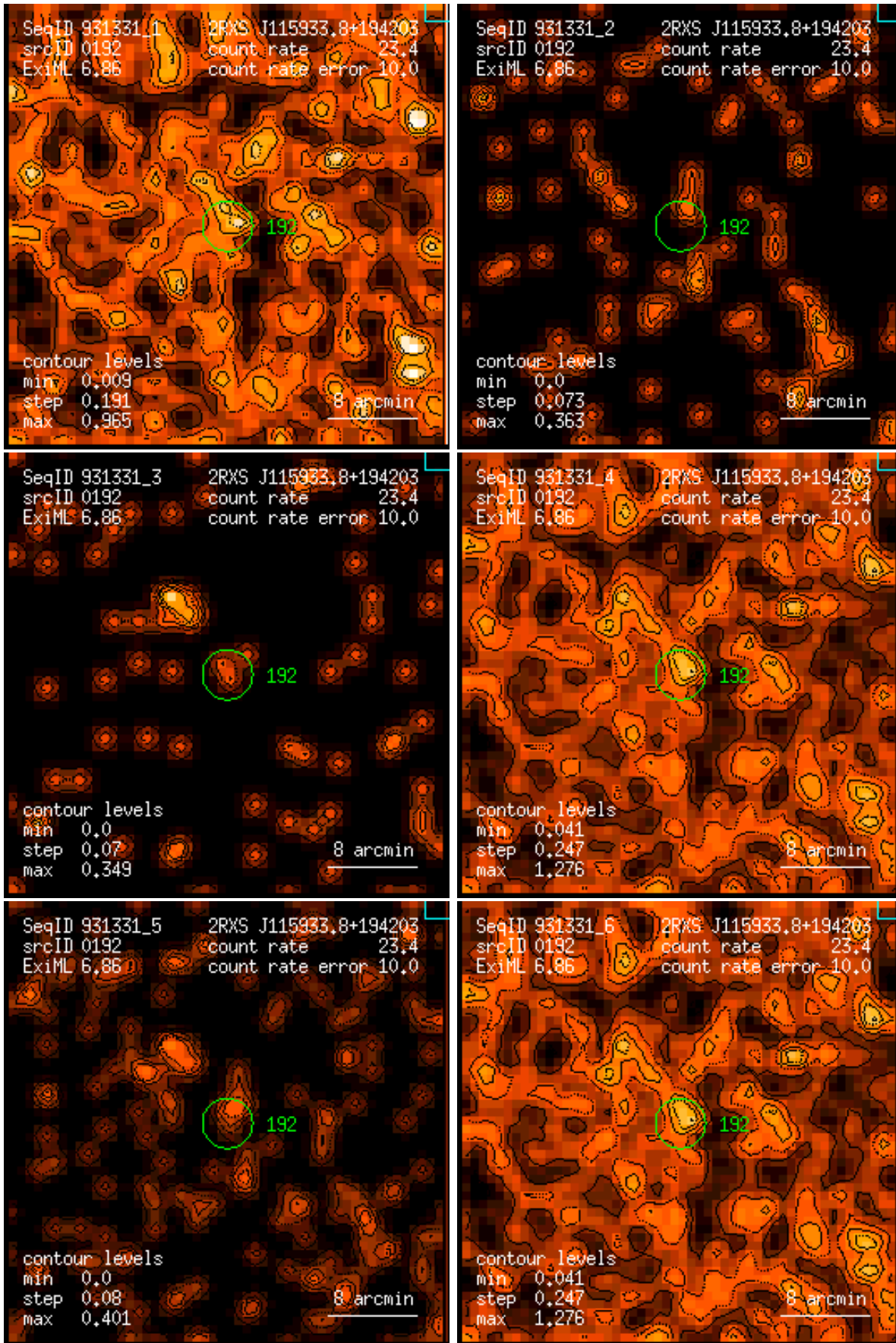
Figure 192: RASS 931331: detection 0192: band rate images, Gaussian filter: (1) PSPC channels 11 – 41, (2) 52 – 90, (3) 91 – 201, (4) 11 – 235, (5) 52 – 201, (6) 11 – 201. Broad band rates in counts/ks. Band rate contour levels in counts/ks/arcmin 2 .
