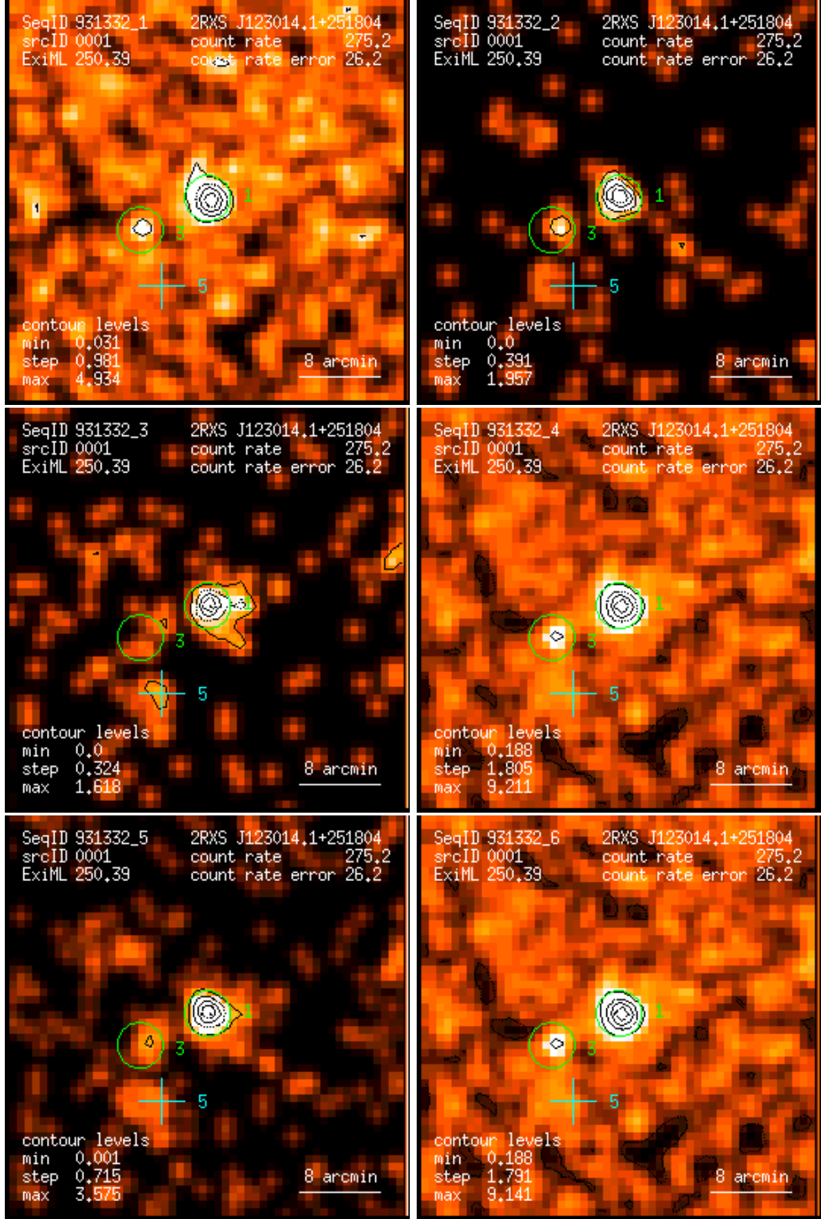
Figure 1: RASS 931332: detection 0001: band rate images, Gaussian filter: (1) PSPC channels 11 – 41, (2) 52 – 90, (3) 91 – 201, (4) 11 – 235, (5) 52 – 201, (6) 11 – 201. Broad band rates in counts/ks. Band rate contour levels in counts/ks/arcmin 2 .
