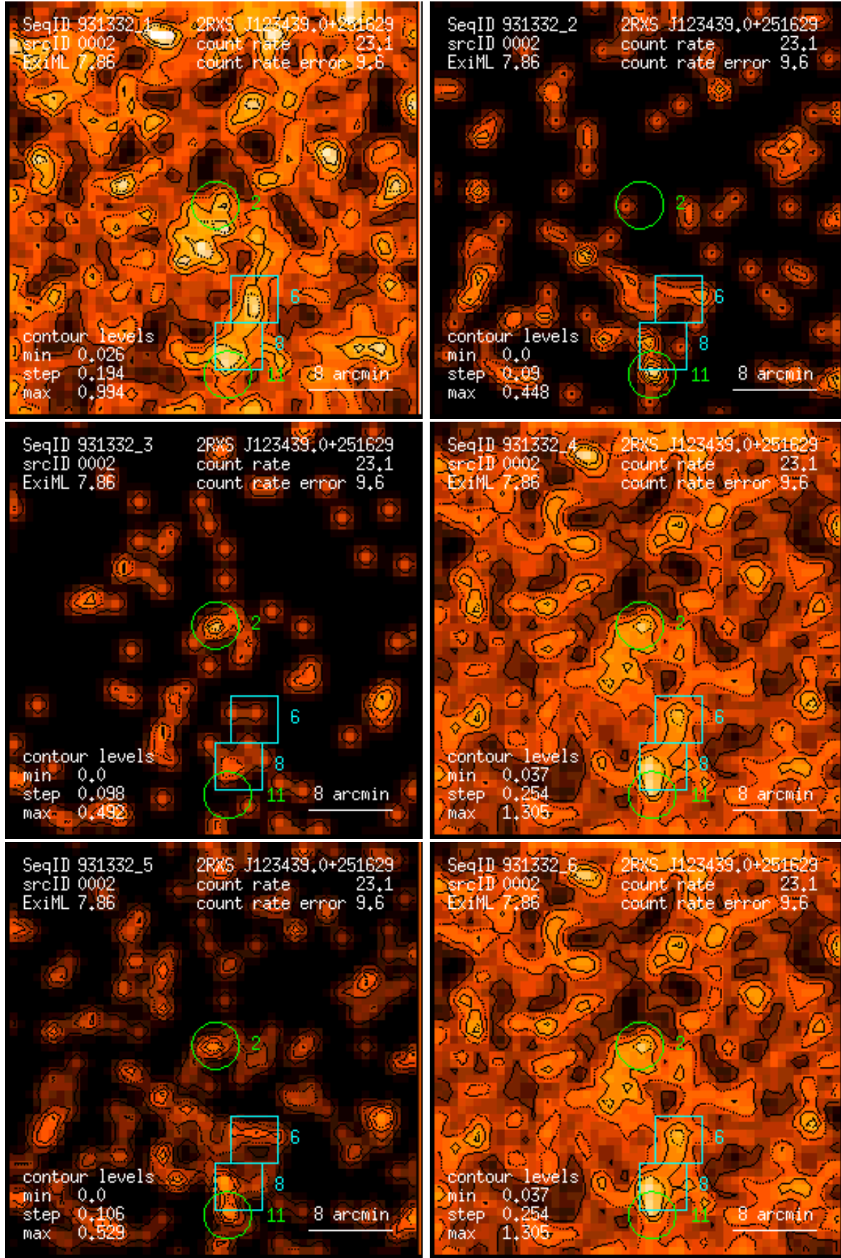
Figure 2: RASS 931332: detection 0002: band rate images, Gaussian filter: (1) PSPC channels 11 – 41, (2) 52 – 90, (3) 91 – 201, (4) 11 – 235, (5) 52 – 201, (6) 11 – 201. Broad band rates in counts/ks. Band rate contour levels in counts/ks/arcmin 2 .
