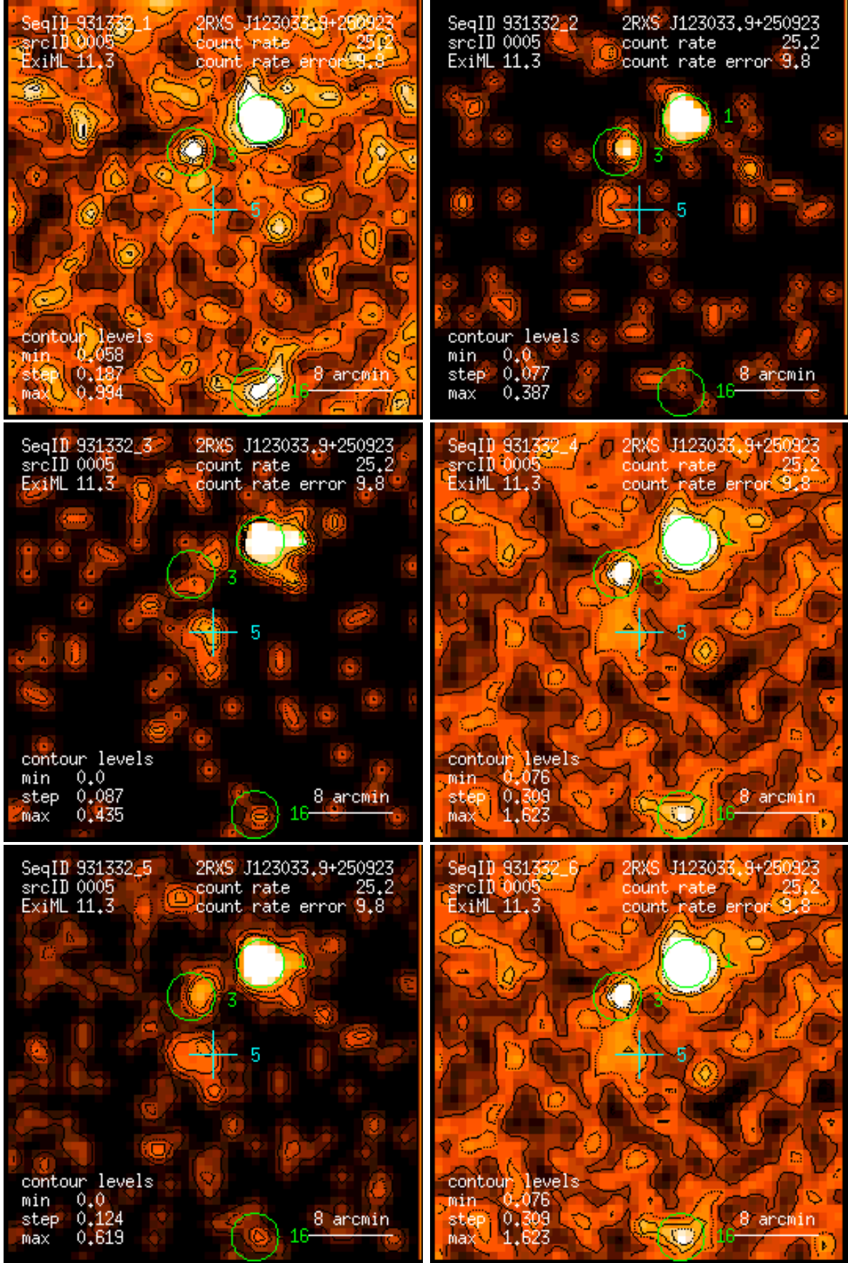
Figure 5: RASS 931332: detection 0005: band rate images, Gaussian filter: (1) PSPC channels 11 – 41, (2) 52 – 90, (3) 91 – 201, (4) 11 – 235, (5) 52 – 201, (6) 11 – 201. Broad band rates in counts/ks. Band rate contour levels in counts/ks/arcmin 2 .
