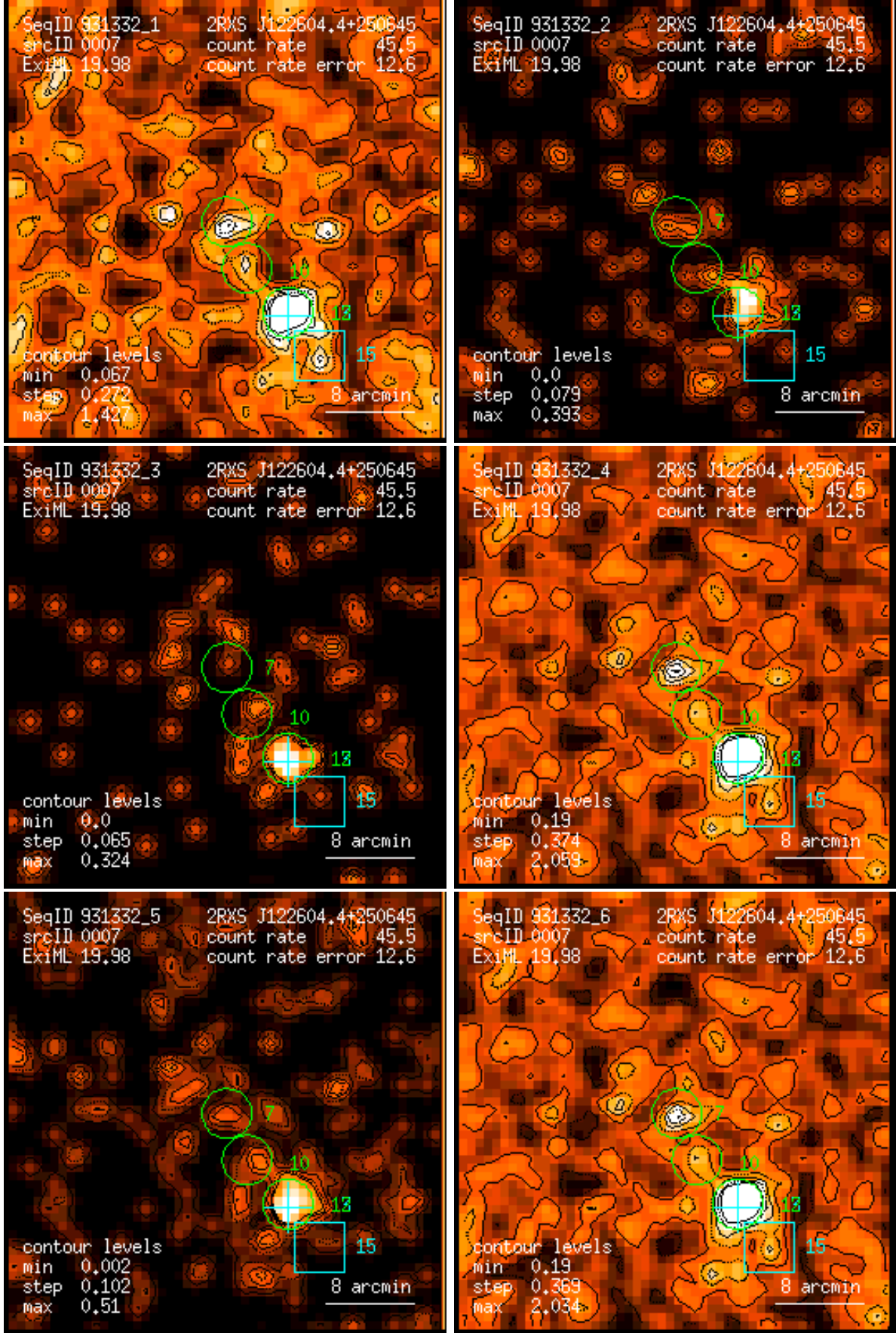
Figure 7: RASS 931332: detection 0007: band rate images, Gaussian filter: (1) PSPC channels 11 – 41, (2) 52 – 90, (3) 91 – 201, (4) 11 – 235, (5) 52 – 201, (6) 11 – 201. Broad band rates in counts/ks. Band rate contour levels in counts/ks/arcmin 2 .
