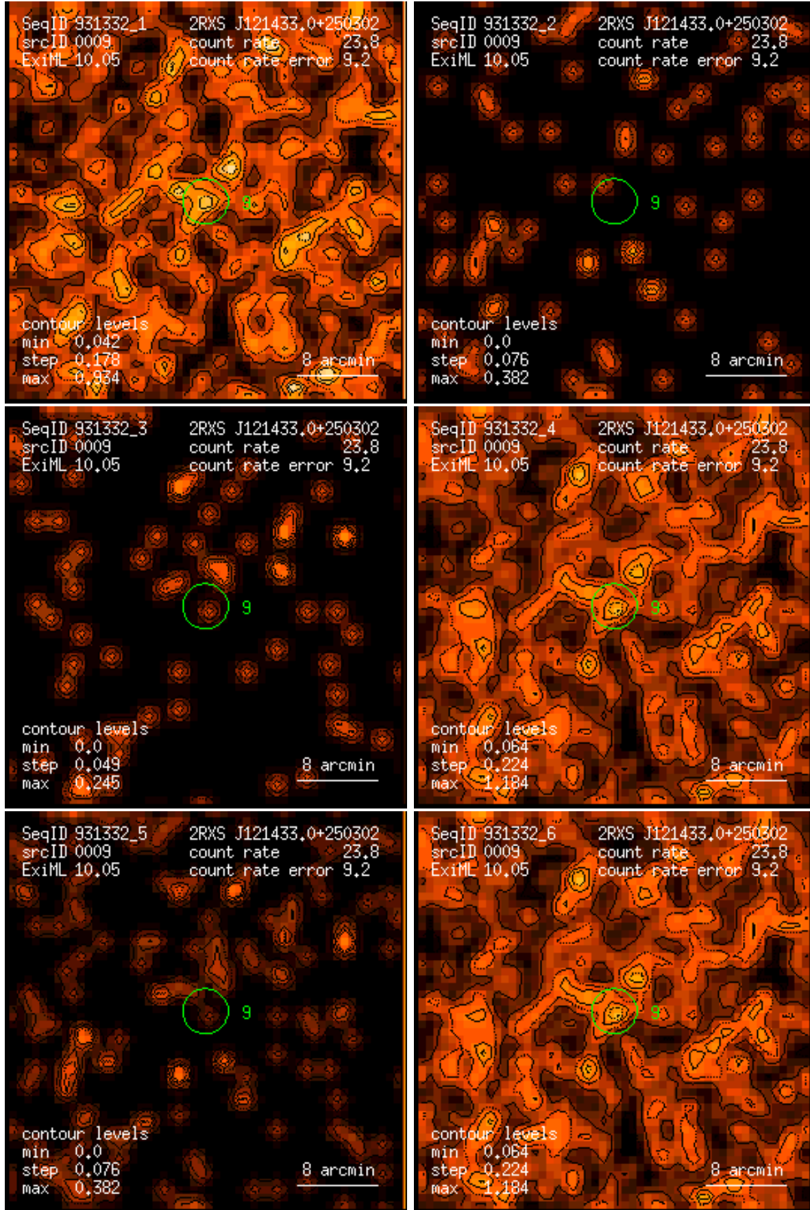
Figure 9: RASS 931332: detection 0009: band rate images, Gaussian filter: (1) PSPC channels 11 – 41, (2) 52 – 90, (3) 91 – 201, (4) 11 – 235, (5) 52 – 201, (6) 11 – 201. Broad band rates in counts/ks. Band rate contour levels in counts/ks/arcmin 2 .
