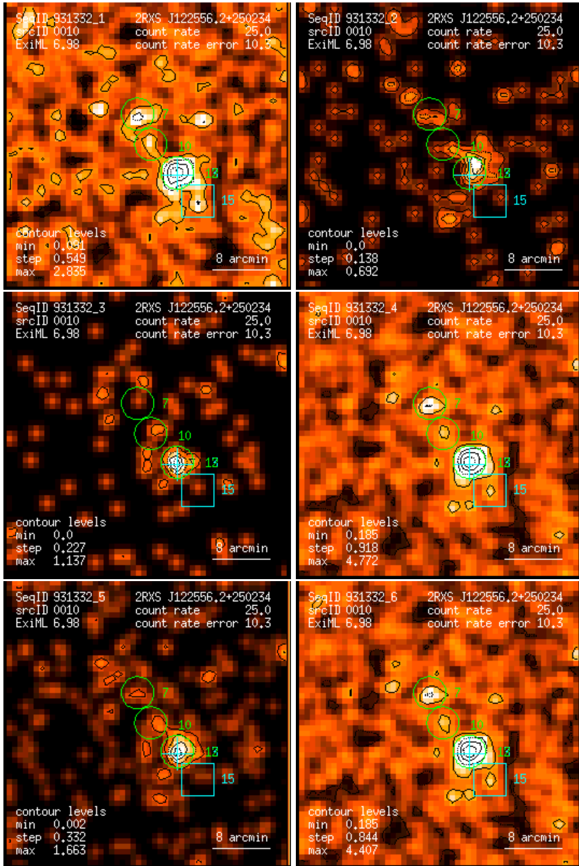
Figure 10: RASS 931332: detection 0010: band rate images, Gaussian filter: (1) PSPC channels 11 – 41, (2) 52 – 90, (3) 91 – 201, (4) 11 – 235, (5) 52 – 201, (6) 11 – 201. Broad band rates in counts/ks. Band rate contour levels in counts/ks/arcmin 2 .
