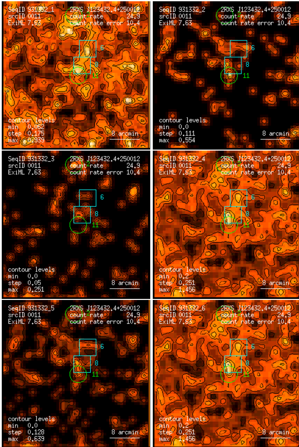
Figure 11: RASS 931332: detection 0011: band rate images, Gaussian filter: (1) PSPC channels 11 – 41, (2) 52 – 90, (3) 91 – 201, (4) 11 – 235, (5) 52 – 201, (6) 11 – 201. Broad band rates in counts/ks. Band rate contour levels in counts/ks/arcmin 2 .
