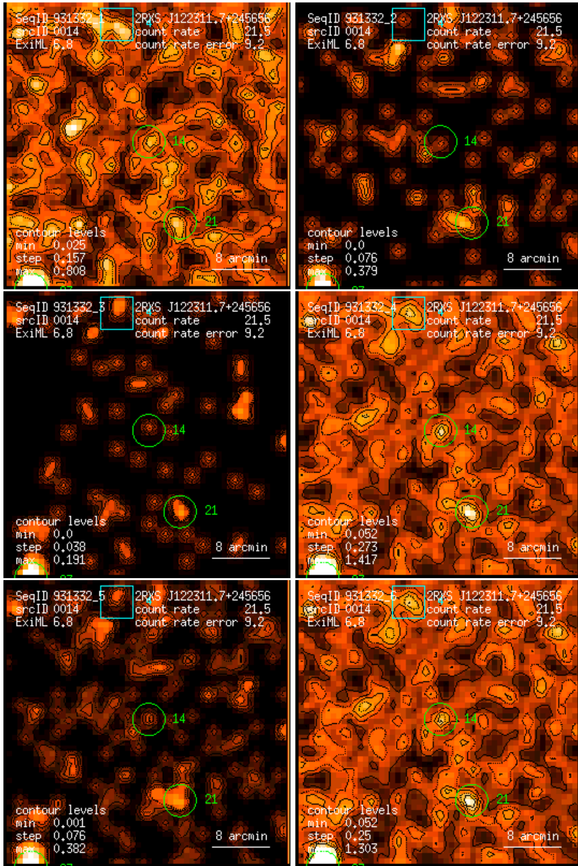
Figure 14: RASS 931332: detection 0014: band rate images, Gaussian filter: (1) PSPC channels 11 – 41, (2) 52 – 90, (3) 91 – 201, (4) 11 – 235, (5) 52 – 201, (6) 11 – 201. Broad band rates in counts/ks. Band rate contour levels in counts/ks/arcmin 2 .
