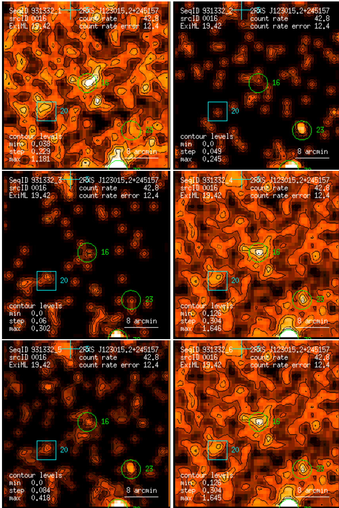
Figure 16: RASS 931332: detection 0016: band rate images, Gaussian filter: (1) PSPC channels 11 – 41, (2) 52 – 90, (3) 91 – 201, (4) 11 – 235, (5) 52 – 201, (6) 11 – 201. Broad band rates in counts/ks. Band rate contour levels in counts/ks/arcmin 2 .
