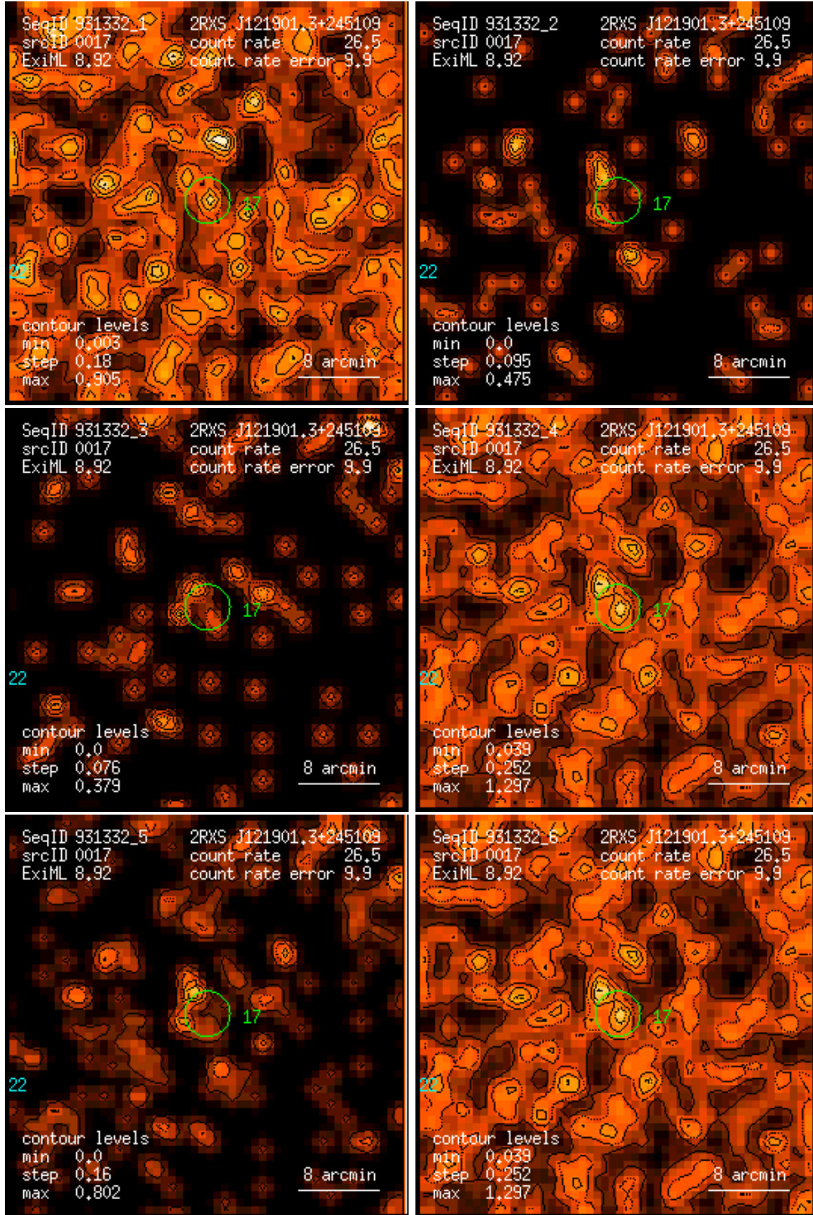
Figure 17: RASS 931332: detection 0017: band rate images, Gaussian filter: (1) PSPC channels 11 – 41, (2) 52 – 90, (3) 91 – 201, (4) 11 – 235, (5) 52 – 201, (6) 11 – 201. Broad band rates in counts/ks. Band rate contour levels in counts/ks/arcmin 2 .
