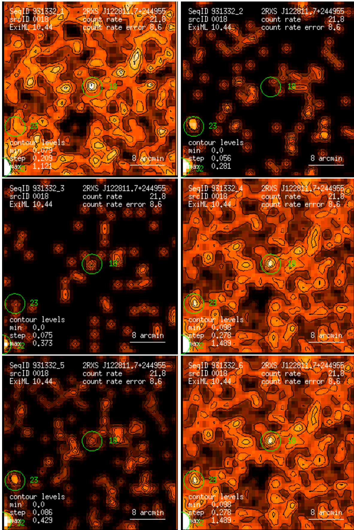
Figure 18: RASS 931332: detection 0018: band rate images, Gaussian filter: (1) PSPC channels 11 – 41, (2) 52 – 90, (3) 91 – 201, (4) 11 – 235, (5) 52 – 201, (6) 11 – 201. Broad band rates in counts/ks. Band rate contour levels in counts/ks/arcmin 2 .
