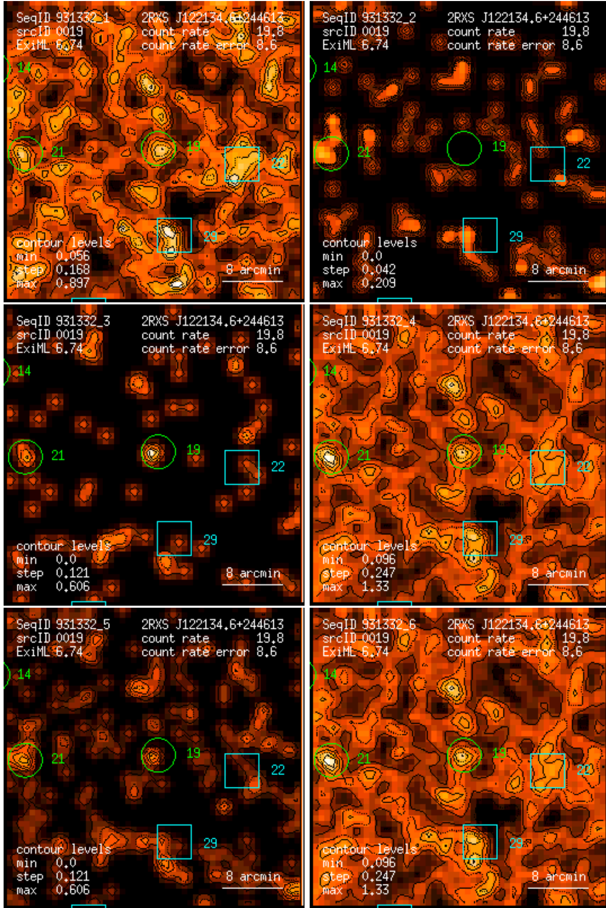
Figure 19: RASS 931332: detection 0019: band rate images, Gaussian filter: (1) PSPC channels 11 – 41, (2) 52 – 90, (3) 91 – 201, (4) 11 – 235, (5) 52 – 201, (6) 11 – 201. Broad band rates in counts/ks. Band rate contour levels in counts/ks/arcmin 2 .
