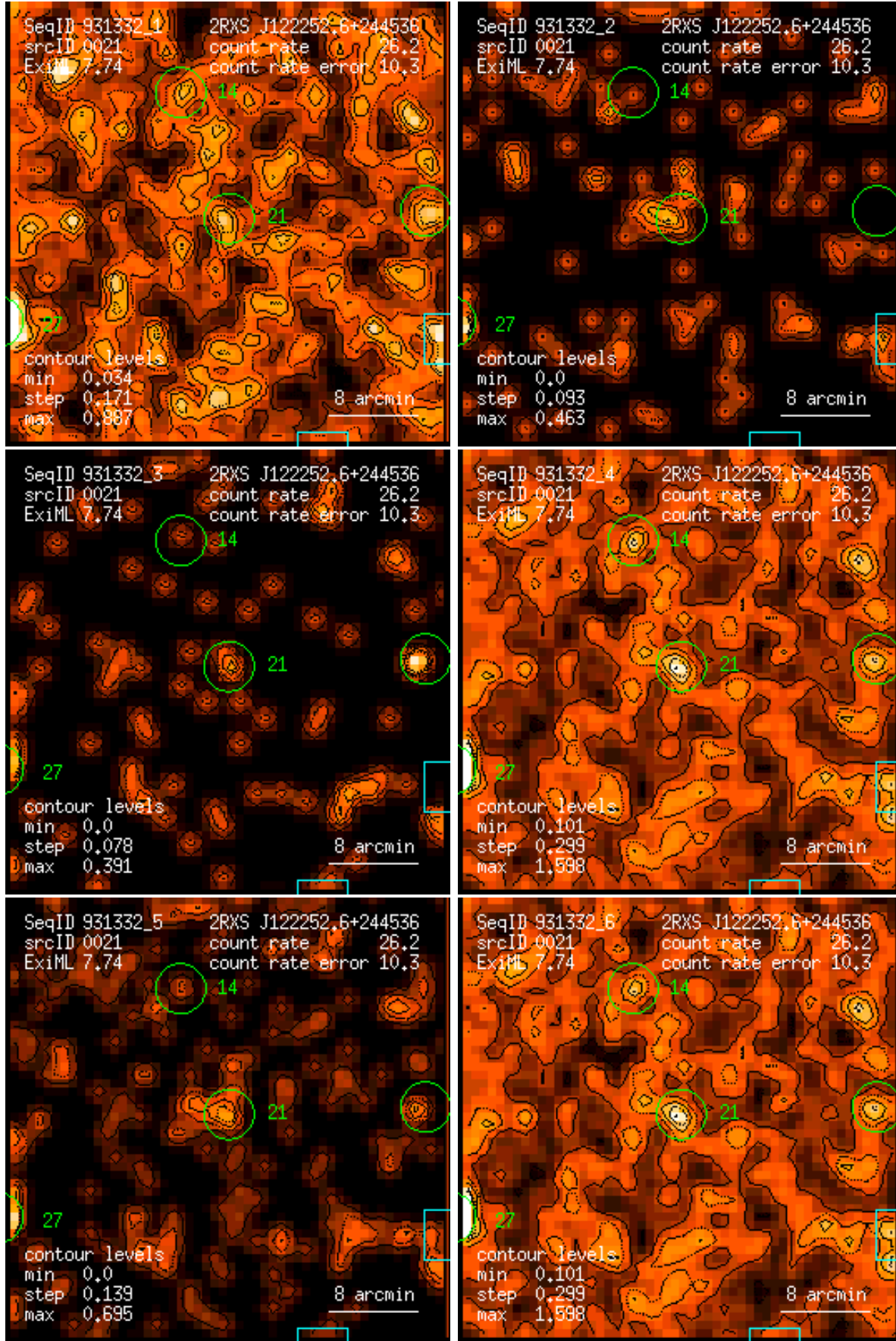
Figure 21: RASS 931332: detection 0021: band rate images, Gaussian filter: (1) PSPC channels 11 – 41, (2) 52 – 90, (3) 91 – 201, (4) 11 – 235, (5) 52 – 201, (6) 11 – 201. Broad band rates in counts/ks. Band rate contour levels in counts/ks/arcmin 2 .
