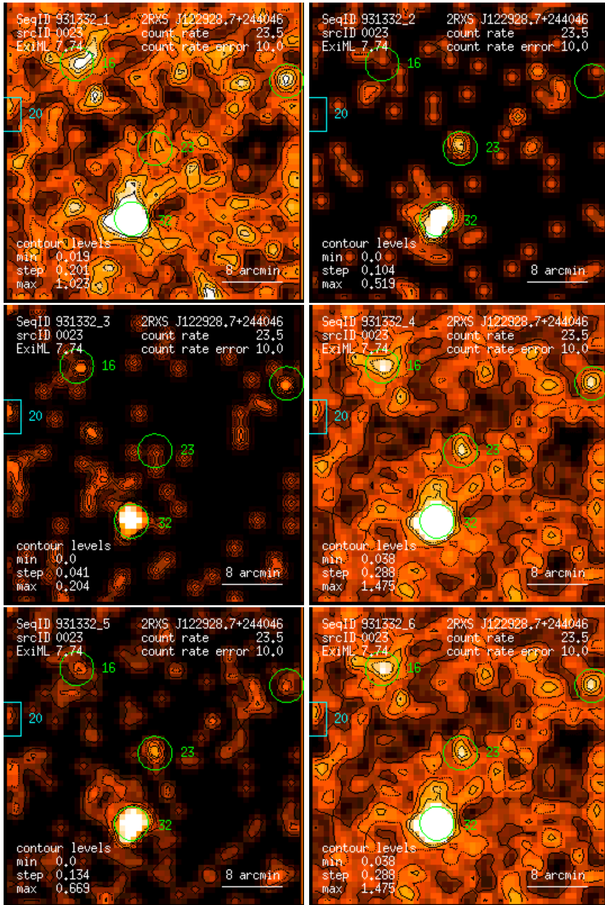
Figure 23: RASS 931332: detection 0023: band rate images, Gaussian filter: (1) PSPC channels 11 – 41, (2) 52 – 90, (3) 91 – 201, (4) 11 – 235, (5) 52 – 201, (6) 11 – 201. Broad band rates in counts/ks. Band rate contour levels in counts/ks/arcmin 2 .
