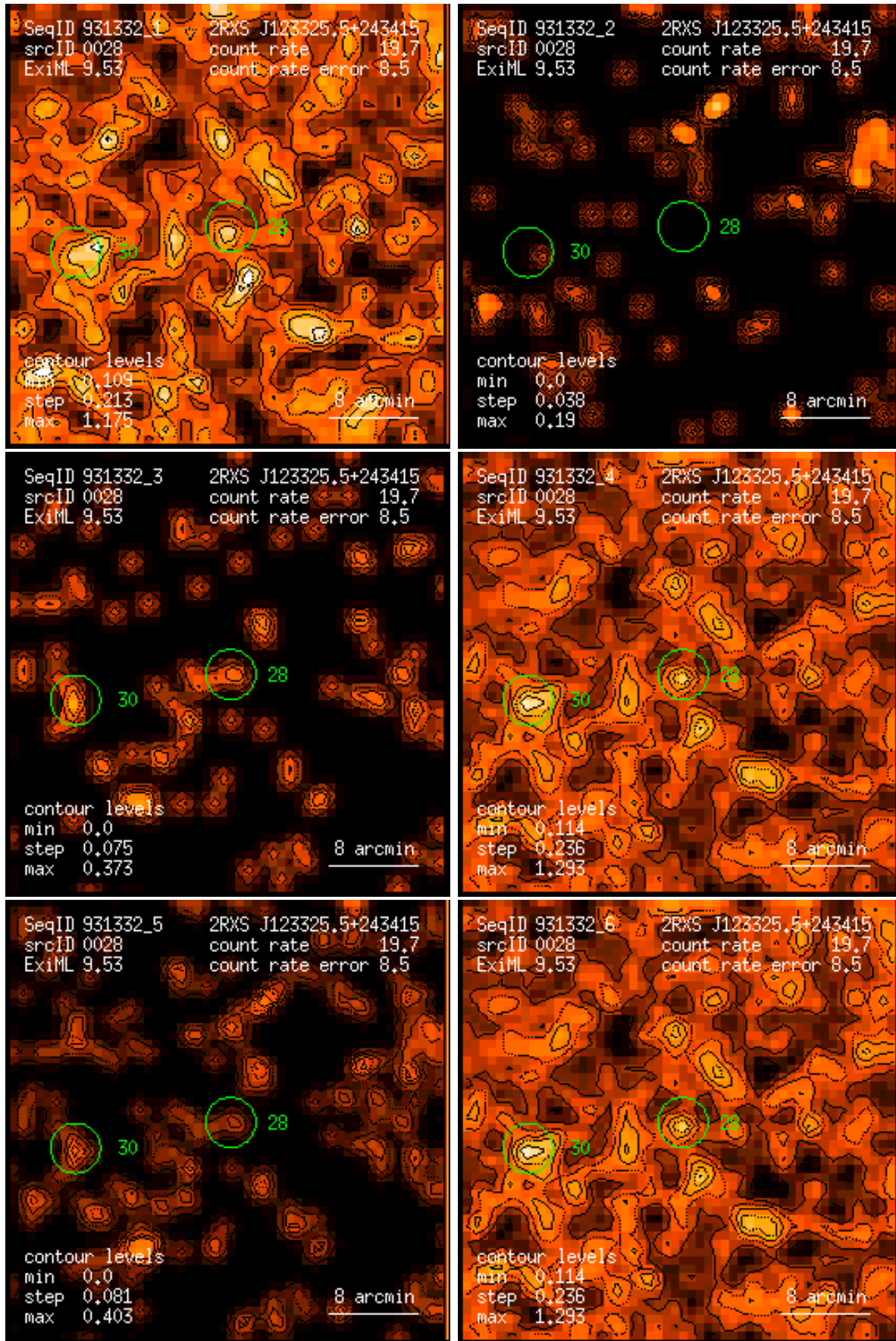
Figure 28: RASS 931332: detection 0028: band rate images, Gaussian filter: (1) PSPC channels 11 – 41, (2) 52 – 90, (3) 91 – 201, (4) 11 – 235, (5) 52 – 201, (6) 11 – 201. Broad band rates in counts/ks. Band rate contour levels in counts/ks/arcmin 2 .
