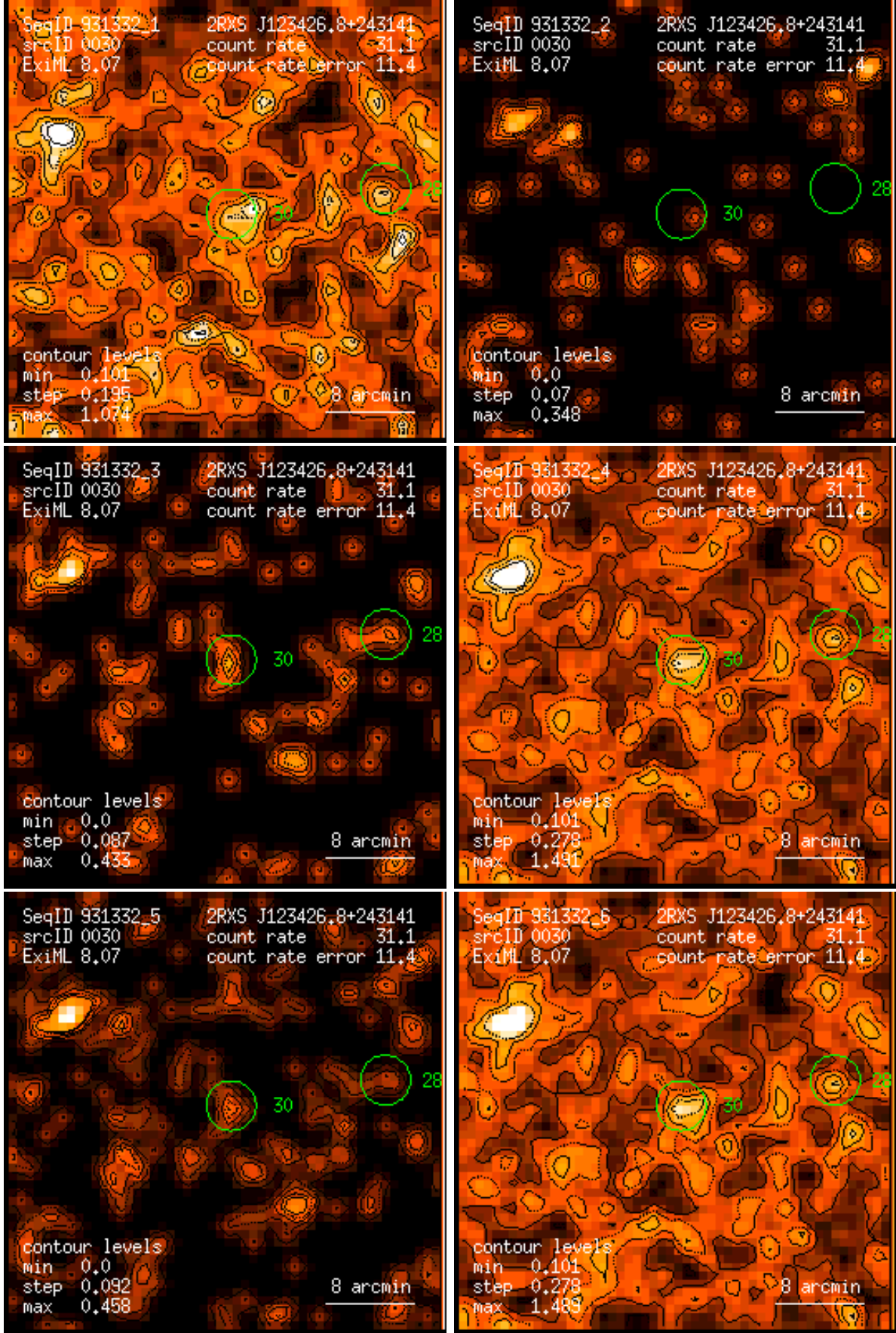
Figure 30: RASS 931332: detection 0030: band rate images, Gaussian filter: (1) PSPC channels 11 – 41, (2) 52 – 90, (3) 91 – 201, (4) 11 – 235, (5) 52 – 201, (6) 11 – 201. Broad band rates in counts/ks. Band rate contour levels in counts/ks/arcmin 2 .
