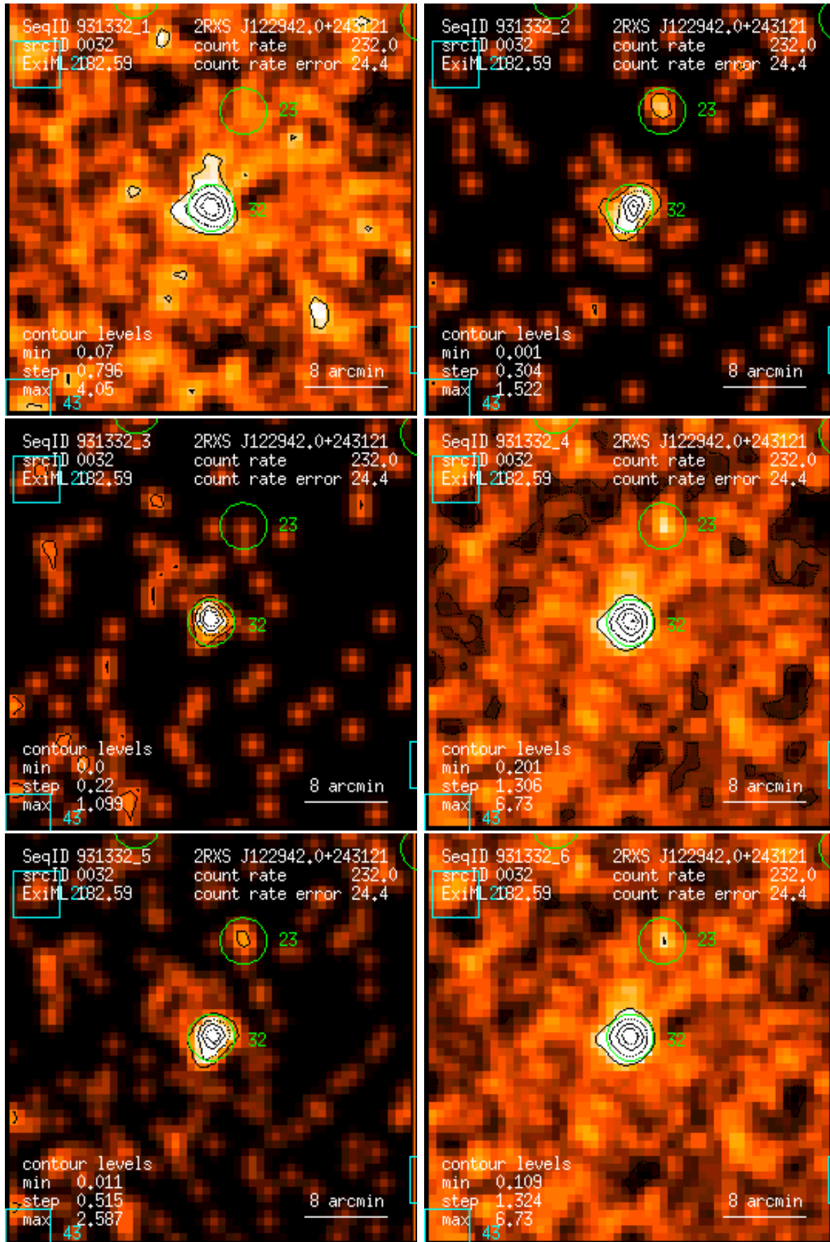
Figure 32: RASS 931332: detection 0032: band rate images, Gaussian filter: (1) PSPC channels 11 – 41, (2) 52 – 90, (3) 91 – 201, (4) 11 – 235, (5) 52 – 201, (6) 11 – 201. Broad band rates in counts/ks. Band rate contour levels in counts/ks/arcmin 2 .
