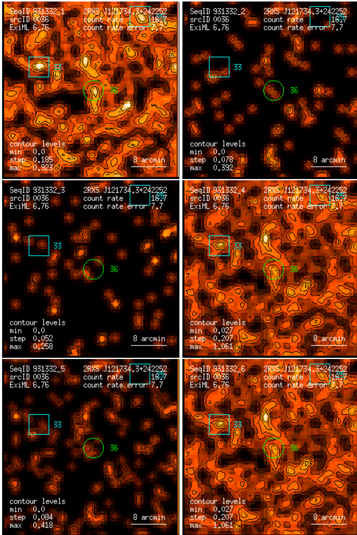
Figure 36: RASS 931332: detection 0036: band rate images, Gaussian filter: (1) PSPC channels 11 – 41, (2) 52 – 90, (3) 91 – 201, (4) 11 – 235, (5) 52 – 201, (6) 11 – 201. Broad band rates in counts/ks. Band rate contour levels in counts/ks/arcmin 2 .
