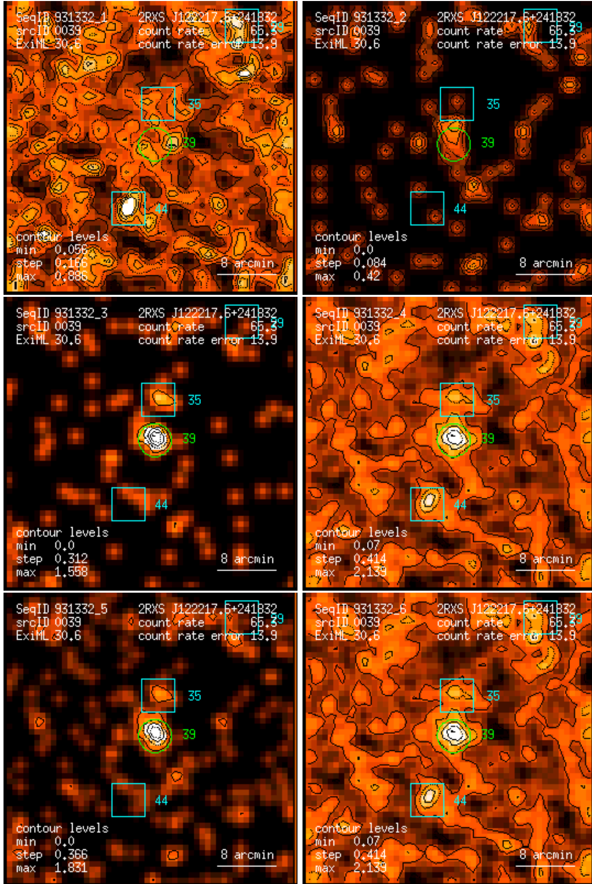
Figure 39: RASS 931332: detection 0039: band rate images, Gaussian filter: (1) PSPC channels 11 – 41, (2) 52 – 90, (3) 91 – 201, (4) 11 – 235, (5) 52 – 201, (6) 11 – 201. Broad band rates in counts/ks. Band rate contour levels in counts/ks/arcmin 2 .
