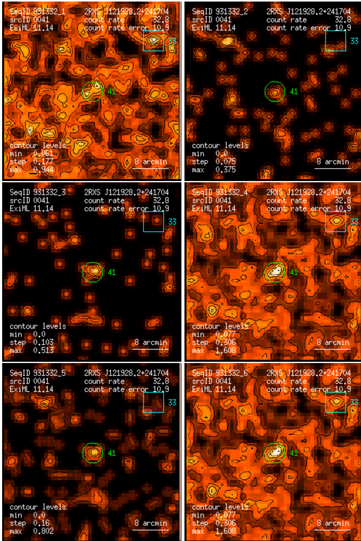
Figure 41: RASS 931332: detection 0041: band rate images, Gaussian filter: (1) PSPC channels 11 – 41, (2) 52 – 90, (3) 91 – 201, (4) 11 – 235, (5) 52 – 201, (6) 11 – 201. Broad band rates in counts/ks. Band rate contour levels in counts/ks/arcmin 2 .
