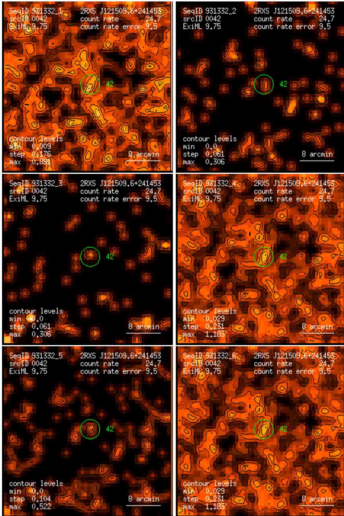
Figure 42: RASS 931332: detection 0042: band rate images, Gaussian filter: (1) PSPC channels 11 – 41, (2) 52 – 90, (3) 91 – 201, (4) 11 – 235, (5) 52 – 201, (6) 11 – 201. Broad band rates in counts/ks. Band rate contour levels in counts/ks/arcmin 2 .
