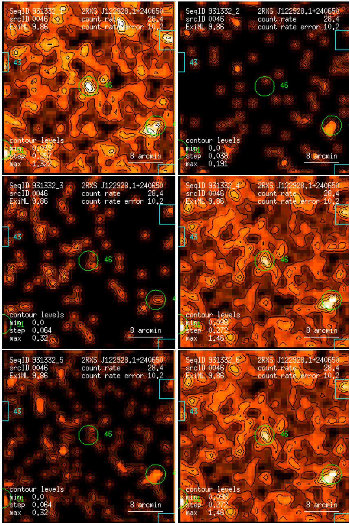
Figure 46: RASS 931332: detection 0046: band rate images, Gaussian filter: (1) PSPC channels 11 – 41, (2) 52 – 90, (3) 91 – 201, (4) 11 – 235, (5) 52 – 201, (6) 11 – 201. Broad band rates in counts/ks. Band rate contour levels in counts/ks/arcmin 2 .
