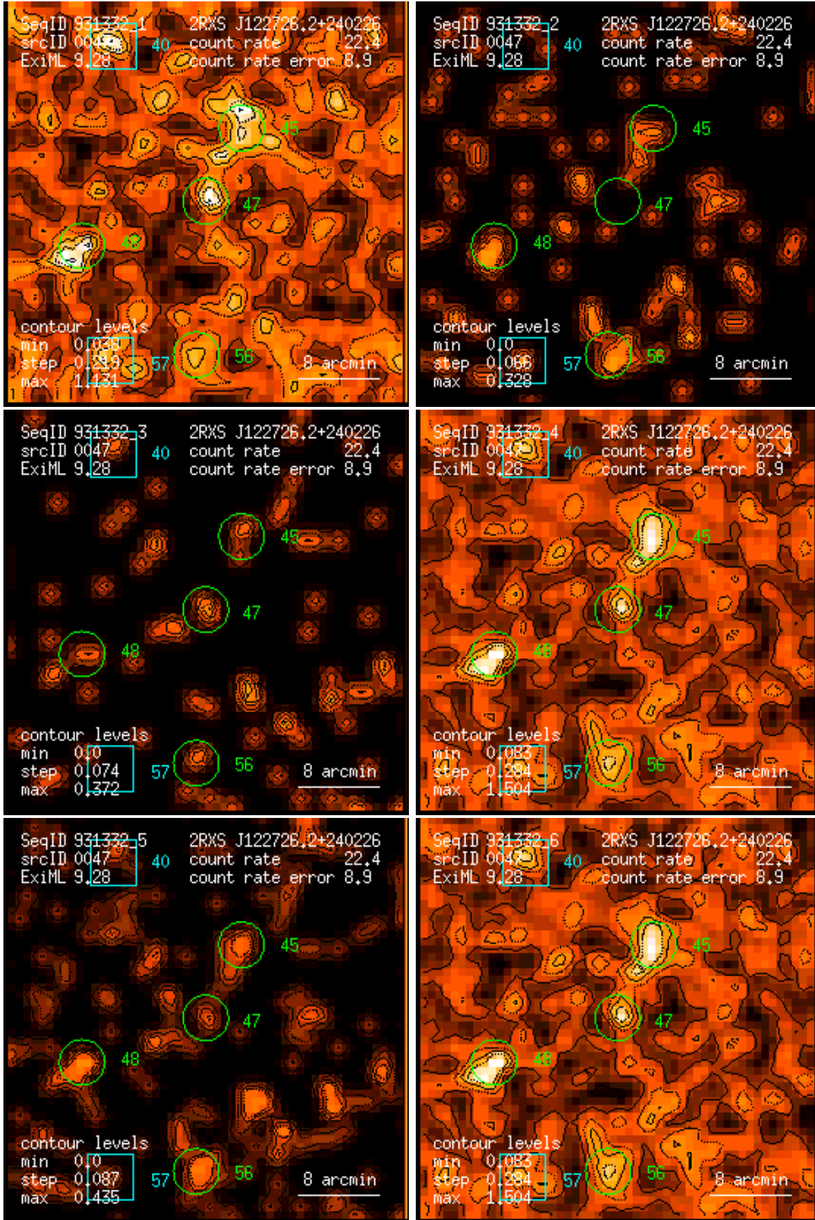
Figure 47: RASS 931332: detection 0047: band rate images, Gaussian filter: (1) PSPC channels 11 – 41, (2) 52 – 90, (3) 91 – 201, (4) 11 – 235, (5) 52 – 201, (6) 11 – 201. Broad band rates in counts/ks. Band rate contour levels in counts/ks/arcmin 2 .
