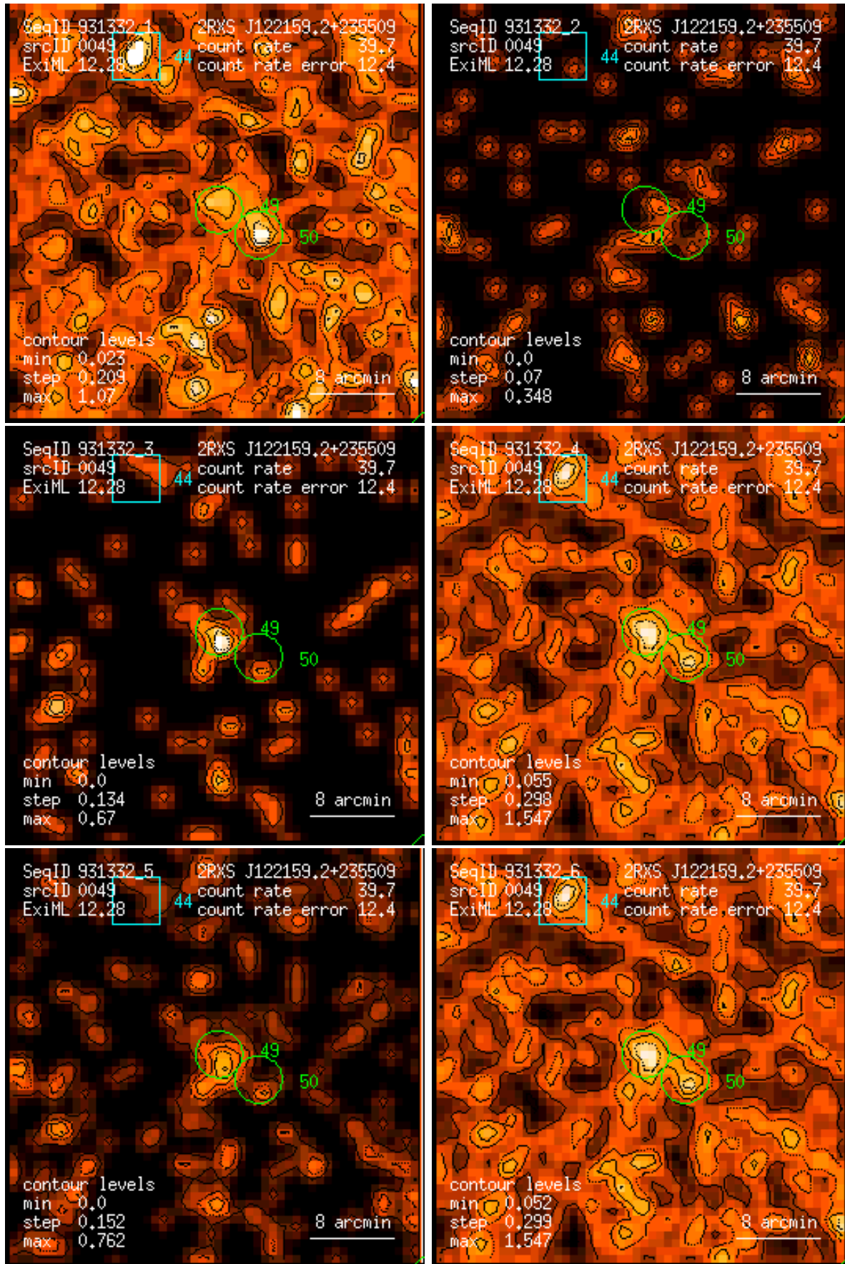
Figure 49: RASS 931332: detection 0049: band rate images, Gaussian filter: (1) PSPC channels 11 – 41, (2) 52 – 90, (3) 91 – 201, (4) 11 – 235, (5) 52 – 201, (6) 11 – 201. Broad band rates in counts/ks. Band rate contour levels in counts/ks/arcmin 2 .
