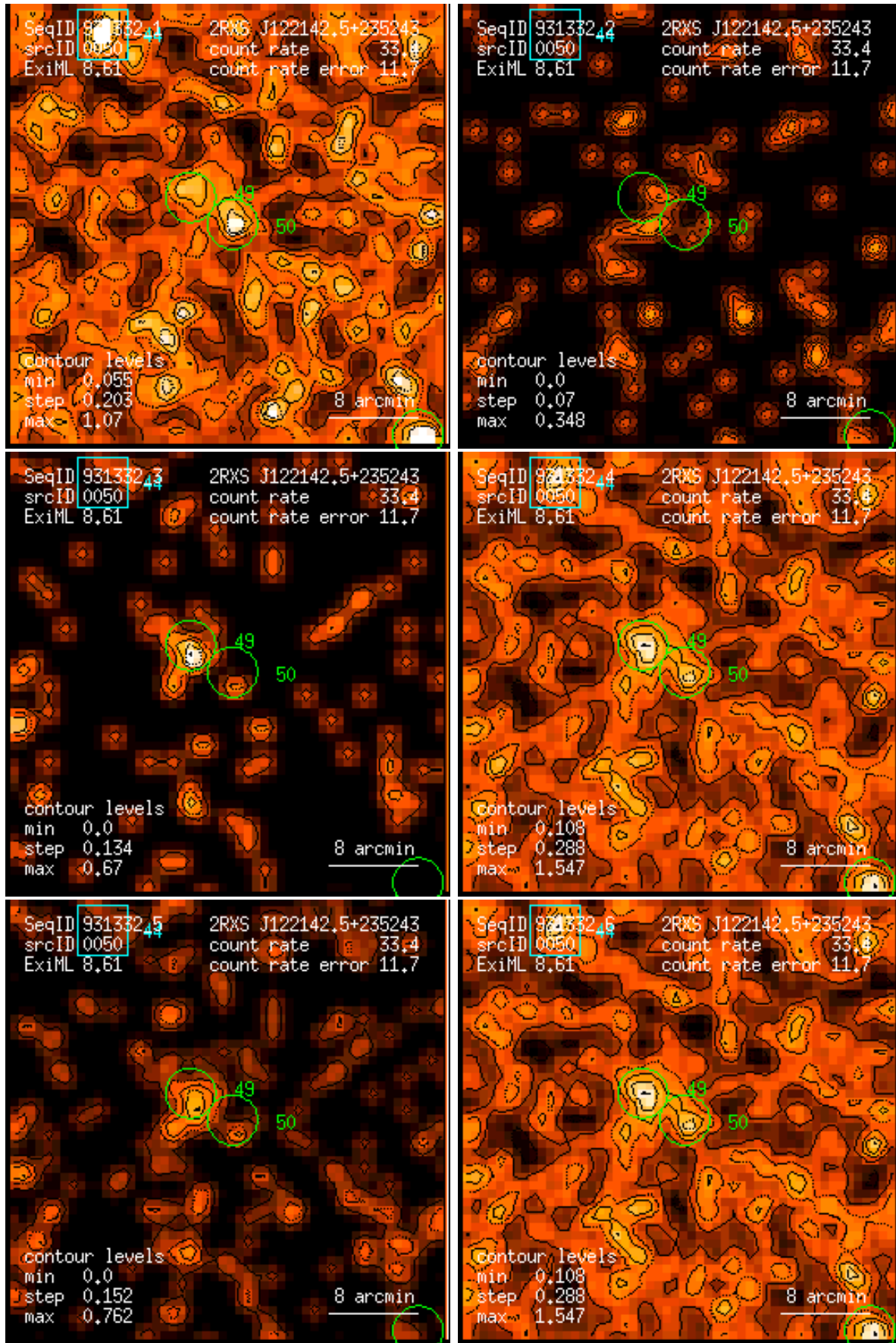
Figure 50: RASS 931332: detection 0050: band rate images, Gaussian filter: (1) PSPC channels 11 – 41, (2) 52 – 90, (3) 91 – 201, (4) 11 – 235, (5) 52 – 201, (6) 11 – 201. Broad band rates in counts/ks. Band rate contour levels in counts/ks/arcmin 2 .
