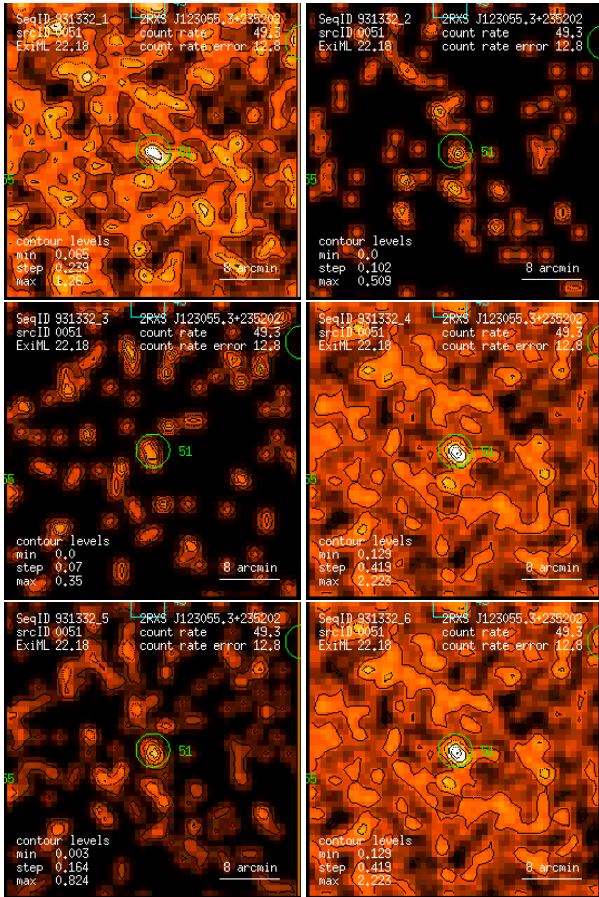
Figure 51: RASS 931332: detection 0051: band rate images, Gaussian filter: (1) PSPC channels 11 – 41, (2) 52 – 90, (3) 91 – 201, (4) 11 – 235, (5) 52 – 201, (6) 11 – 201. Broad band rates in counts/ks. Band rate contour levels in counts/ks/arcmin 2 .
