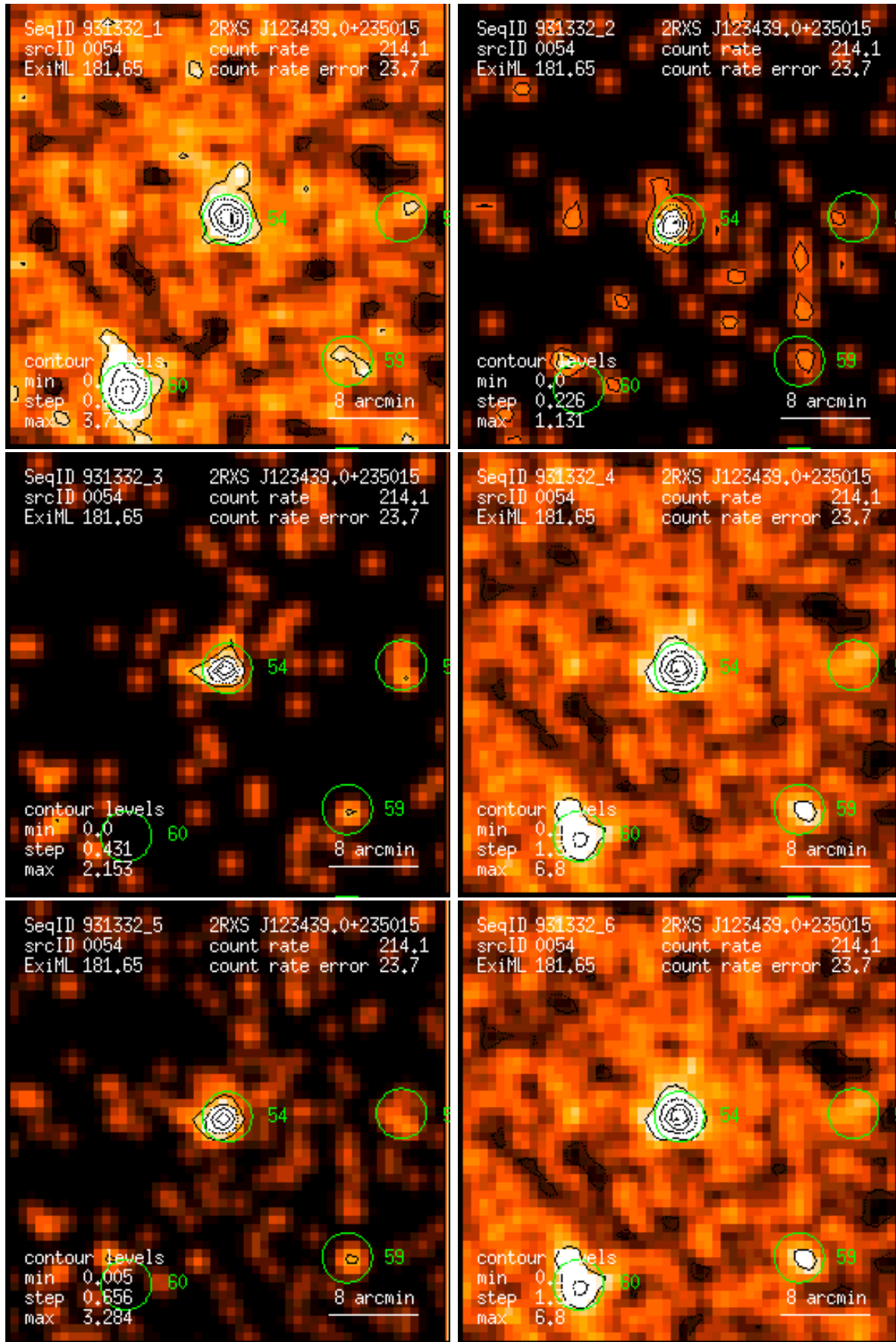
Figure 54: RASS 931332: detection 0054: band rate images, Gaussian filter: (1) PSPC channels 11 – 41, (2) 52 – 90, (3) 91 – 201, (4) 11 – 235, (5) 52 – 201, (6) 11 – 201. Broad band rates in counts/ks. Band rate contour levels in counts/ks/arcmin 2 .
