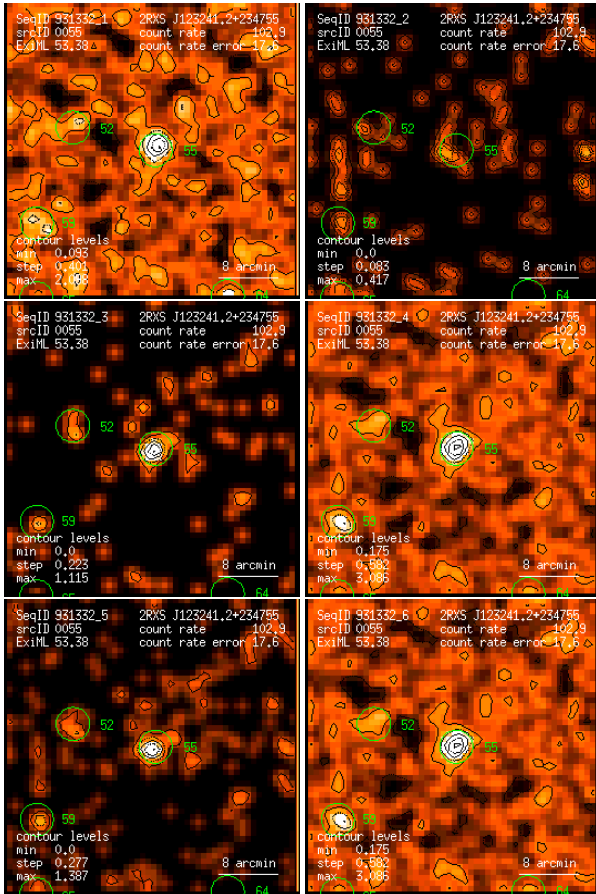
Figure 55: RASS 931332: detection 0055: band rate images, Gaussian filter: (1) PSPC channels 11 – 41, (2) 52 – 90, (3) 91 – 201, (4) 11 – 235, (5) 52 – 201, (6) 11 – 201. Broad band rates in counts/ks. Band rate contour levels in counts/ks/arcmin 2 .
