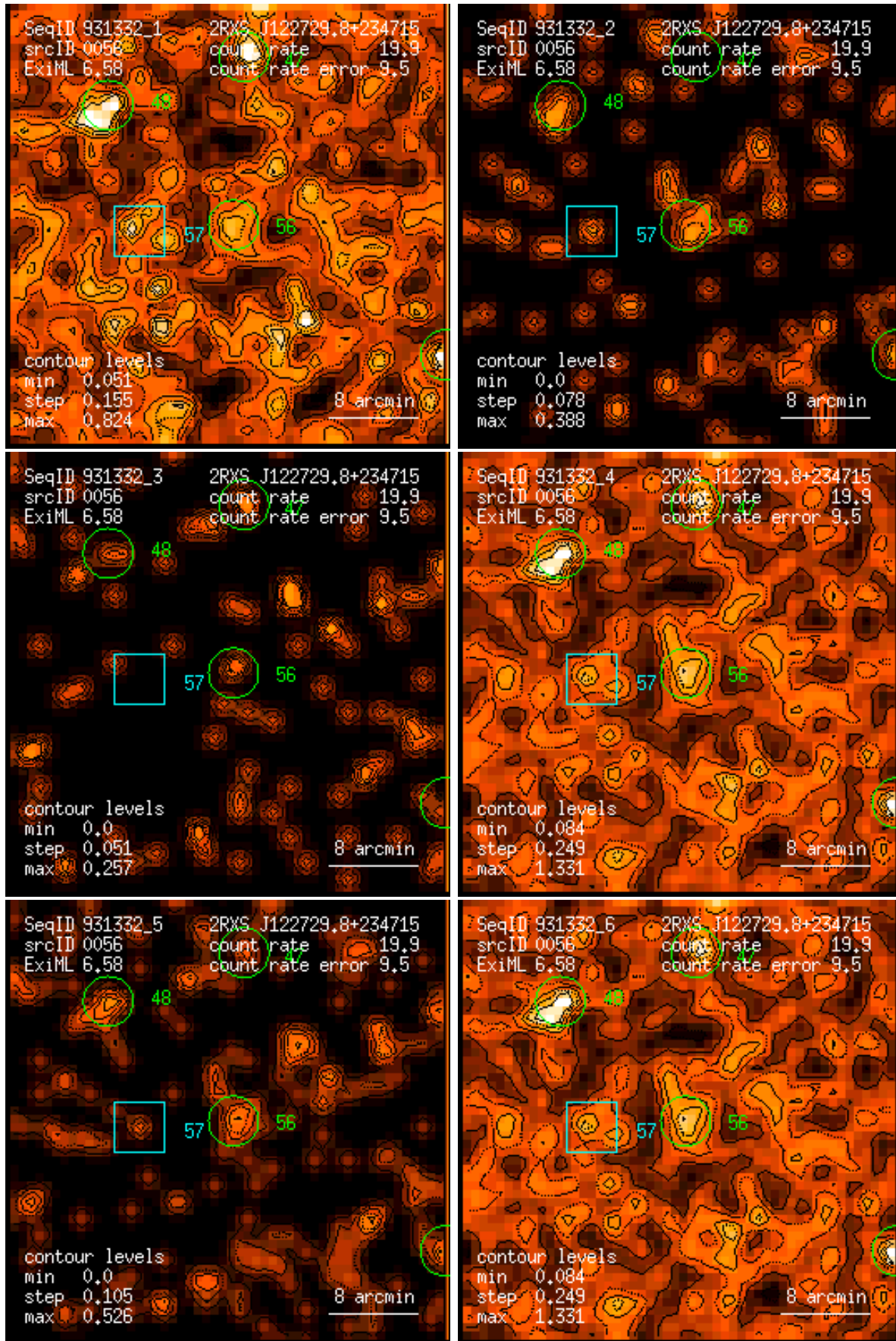
Figure 56: RASS 931332: detection 0056: band rate images, Gaussian filter: (1) PSPC channels 11 – 41, (2) 52 – 90, (3) 91 – 201, (4) 11 – 235, (5) 52 – 201, (6) 11 – 201. Broad band rates in counts/ks. Band rate contour levels in counts/ks/arcmin 2 .
