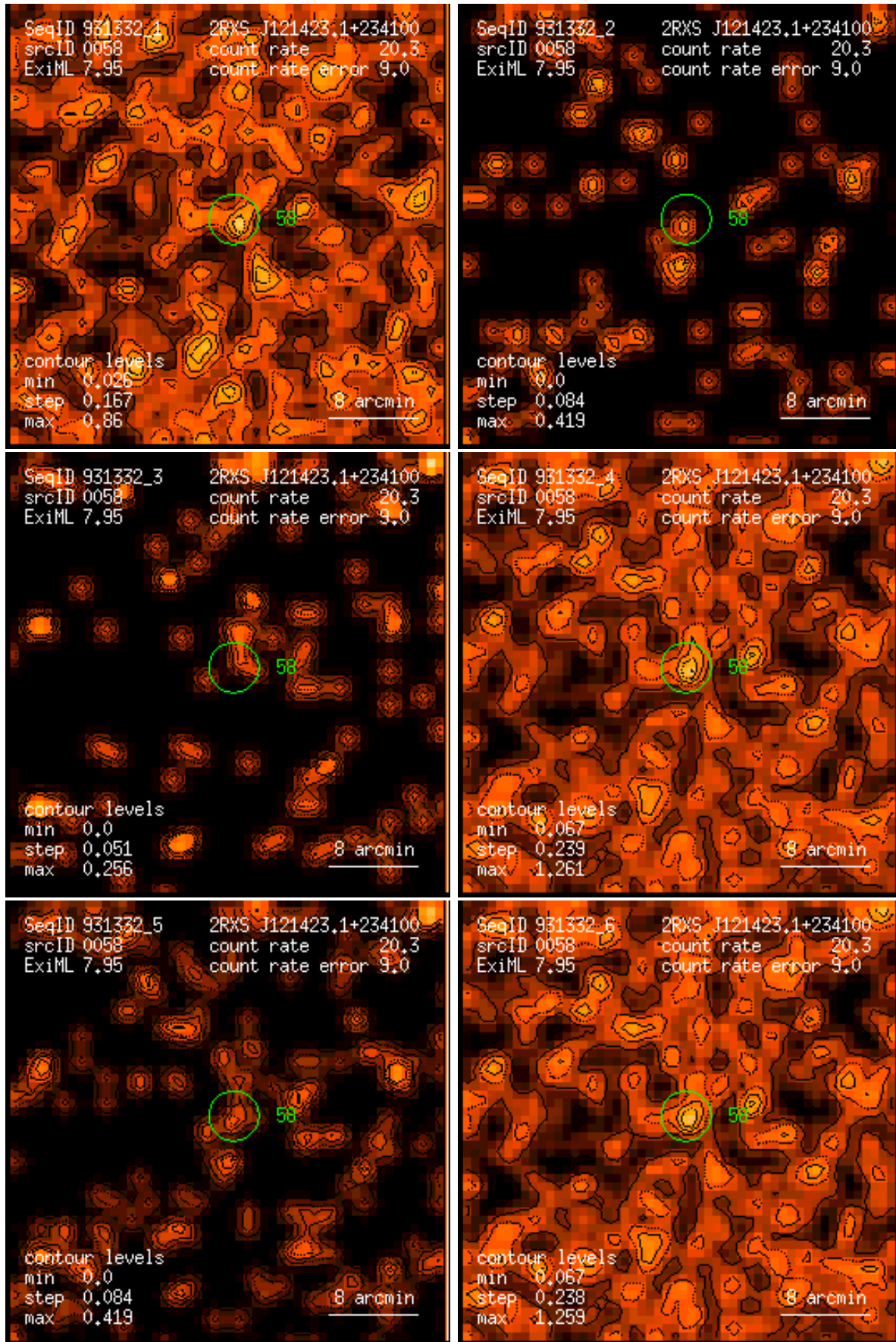
Figure 58: RASS 931332: detection 0058: band rate images, Gaussian filter: (1) PSPC channels 11 – 41, (2) 52 – 90, (3) 91 – 201, (4) 11 – 235, (5) 52 – 201, (6) 11 – 201. Broad band rates in counts/ks. Band rate contour levels in counts/ks/arcmin 2 .
