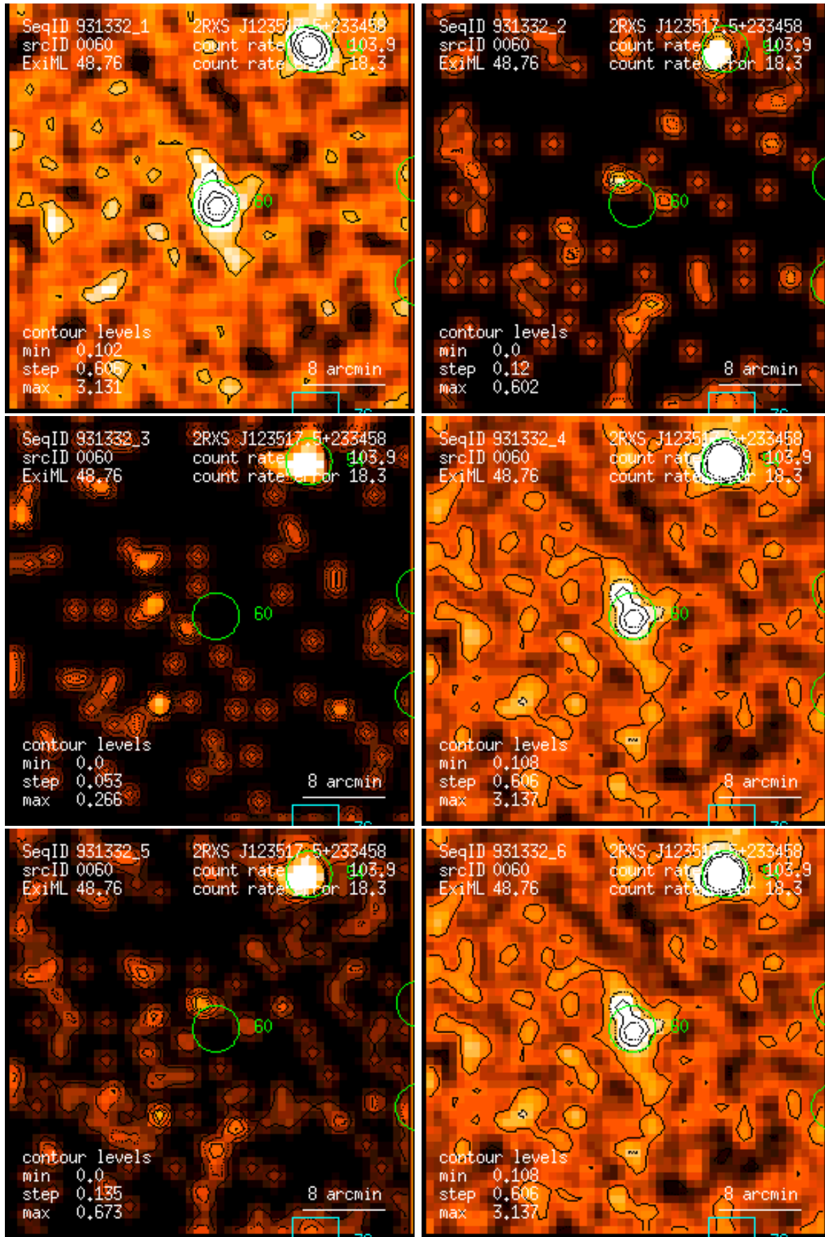
Figure 60: RASS 931332: detection 0060: band rate images, Gaussian filter: (1) PSPC channels 11 – 41, (2) 52 – 90, (3) 91 – 201, (4) 11 – 235, (5) 52 – 201, (6) 11 – 201. Broad band rates in counts/ks. Band rate contour levels in counts/ks/arcmin 2 .
