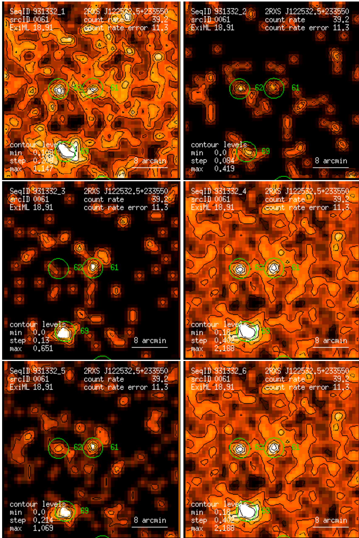
Figure 61: RASS 931332: detection 0061: band rate images, Gaussian filter: (1) PSPC channels 11 – 41, (2) 52 – 90, (3) 91 – 201, (4) 11 – 235, (5) 52 – 201, (6) 11 – 201. Broad band rates in counts/ks. Band rate contour levels in counts/ks/arcmin 2 .
