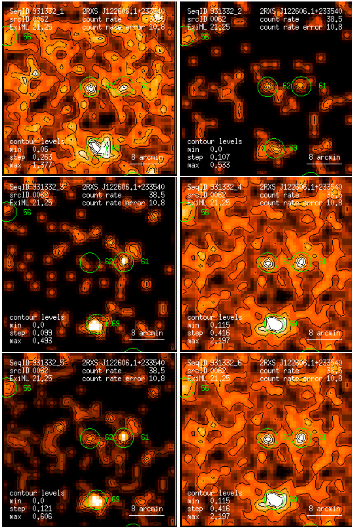
Figure 62: RASS 931332: detection 0062: band rate images, Gaussian filter: (1) PSPC channels 11 – 41, (2) 52 – 90, (3) 91 – 201, (4) 11 – 235, (5) 52 – 201, (6) 11 – 201. Broad band rates in counts/ks. Band rate contour levels in counts/ks/arcmin 2 .
