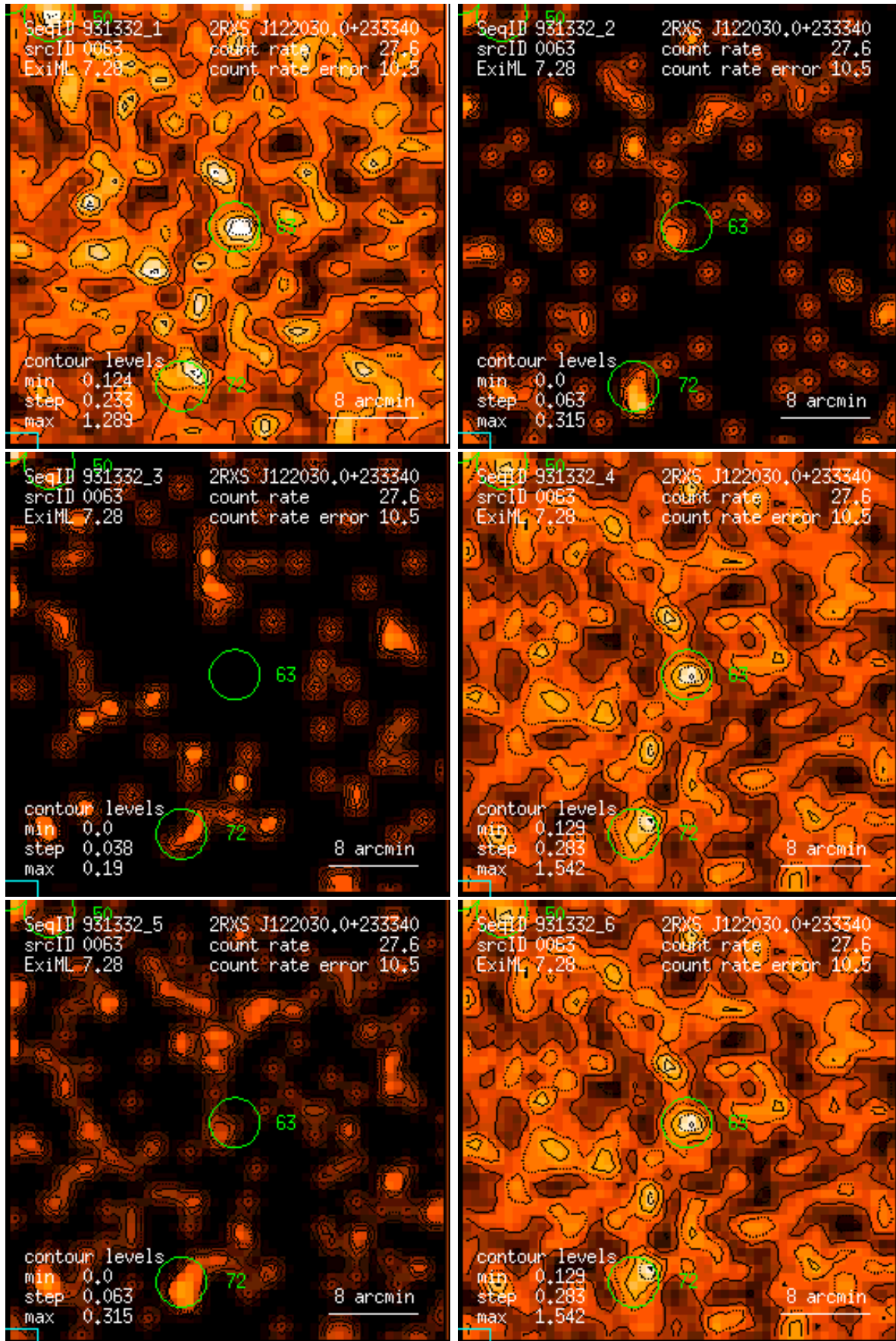
Figure 63: RASS 931332: detection 0063: band rate images, Gaussian filter: (1) PSPC channels 11 – 41, (2) 52 – 90, (3) 91 – 201, (4) 11 – 235, (5) 52 – 201, (6) 11 – 201. Broad band rates in counts/ks. Band rate contour levels in counts/ks/arcmin 2 .
