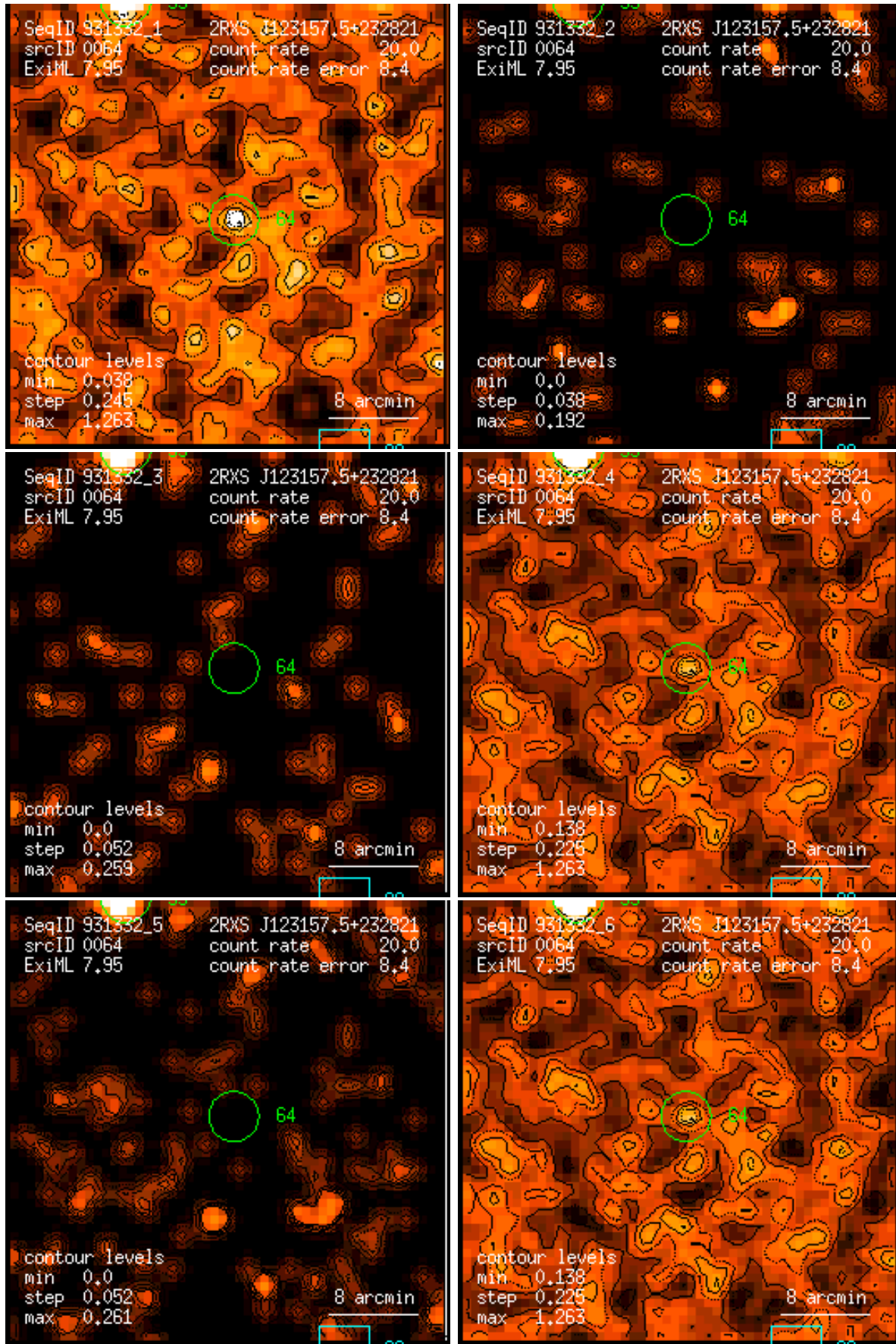
Figure 64: RASS 931332: detection 0064: band rate images, Gaussian filter: (1) PSPC channels 11 – 41, (2) 52 – 90, (3) 91 – 201, (4) 11 – 235, (5) 52 – 201, (6) 11 – 201. Broad band rates in counts/ks. Band rate contour levels in counts/ks/arcmin 2 .
