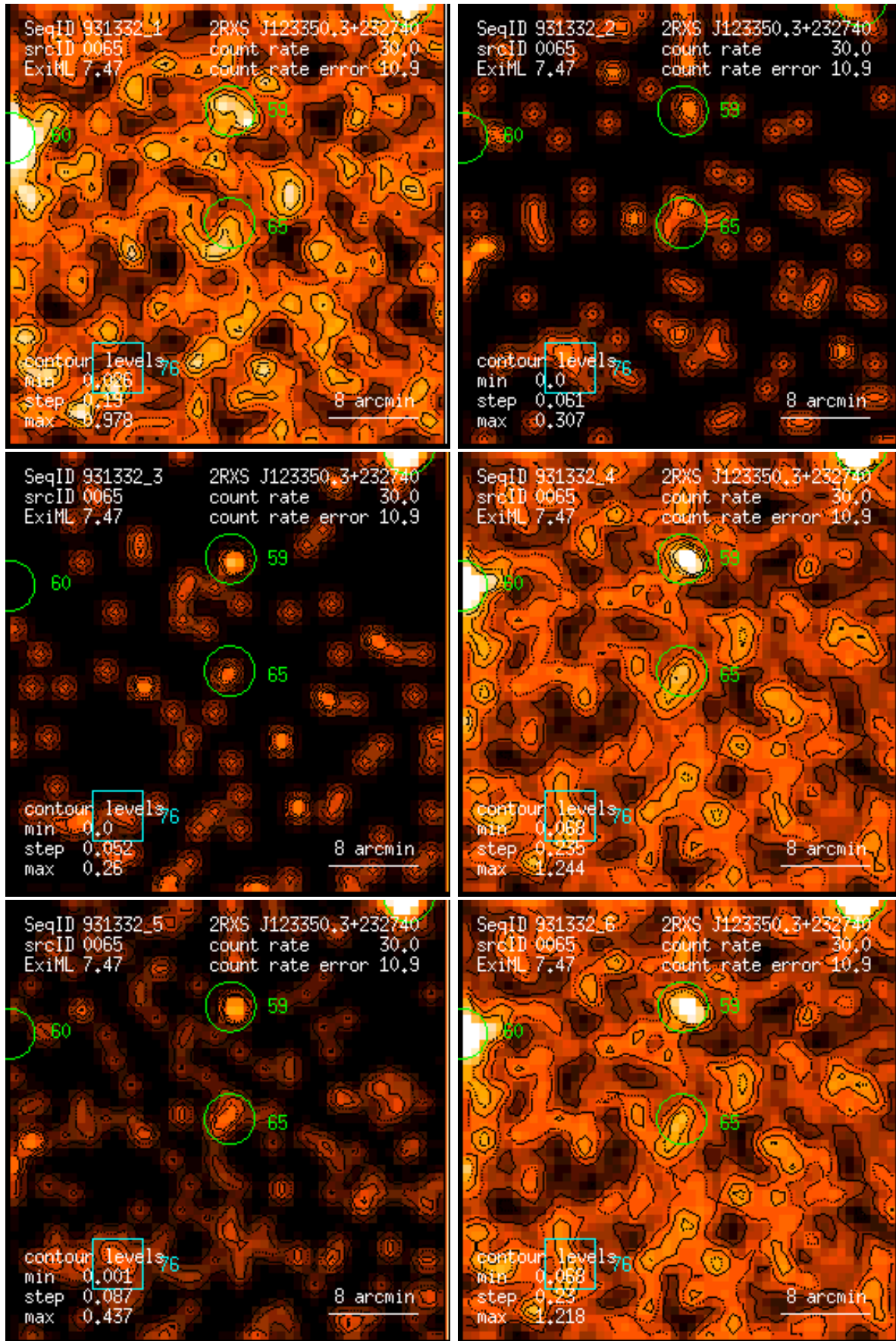
Figure 65: RASS 931332: detection 0065: band rate images, Gaussian filter: (1) PSPC channels 11 – 41, (2) 52 – 90, (3) 91 – 201, (4) 11 – 235, (5) 52 – 201, (6) 11 – 201. Broad band rates in counts/ks. Band rate contour levels in counts/ks/arcmin 2 .
