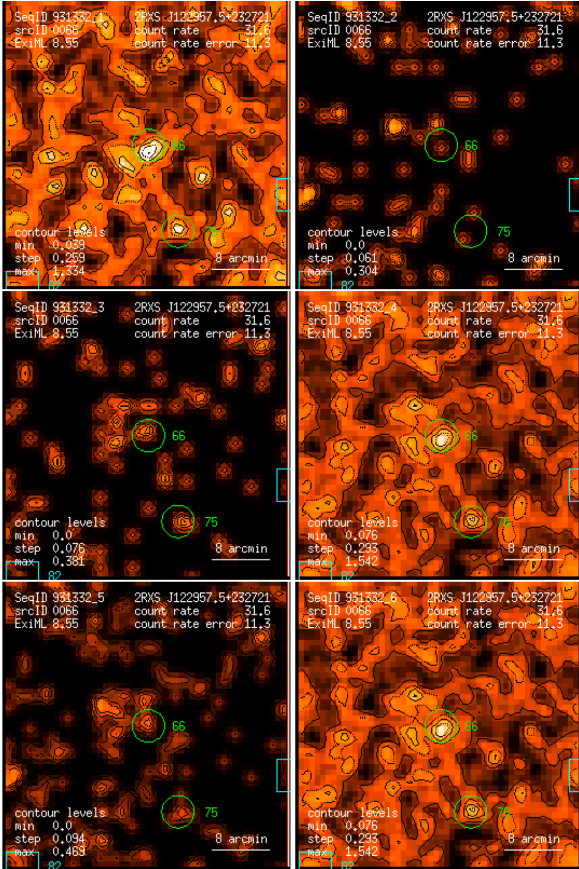
Figure 66: RASS 931332: detection 0066: band rate images, Gaussian filter: (1) PSPC channels 11 – 41, (2) 52 – 90, (3) 91 – 201, (4) 11 – 235, (5) 52 – 201, (6) 11 – 201. Broad band rates in counts/ks. Band rate contour levels in counts/ks/arcmin 2 .
